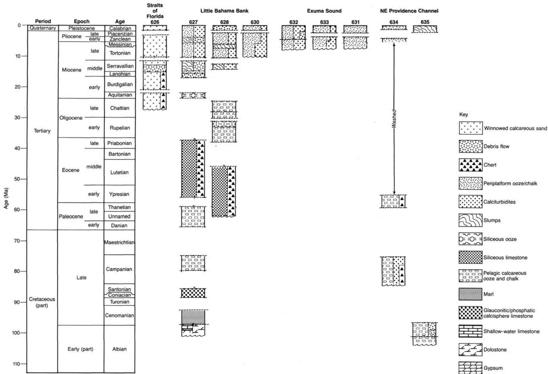
Stratigraphic summary of Leg 101 sites with recovered lithologies plotted according to age. Hiatuses are indicated by wavy horizontal lines. Compiled by R. M. Leckie from data in Austin, Schlager, et al. (1986).
