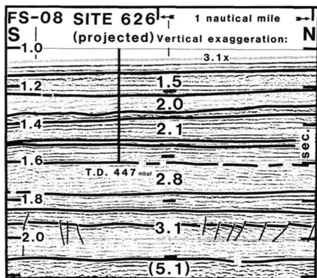
Figure 3. Part of interpreted site-survey profile FS-08 in the vicinity of Site 626 (see Fig. 2 for location). Larger numbers vertically arranged in the center of the profile represent interval velocities in km/s derived from sonobuoy and MCS results (see Austin et al., this volume). Vertical bar represents the total depth (TD) of penetration of Hole 626D in meters. Hole 626D was actually located approximately 0.5 km off the trend of the profile (see Fig. 2 and Austin, Schlager, et al., 1986). Velocity contrast from 3.1 to 5.1 km/s represents the intended drilling target, the inferred top of a mid-Cretaceous(?) shallow-water carbonate platform.
