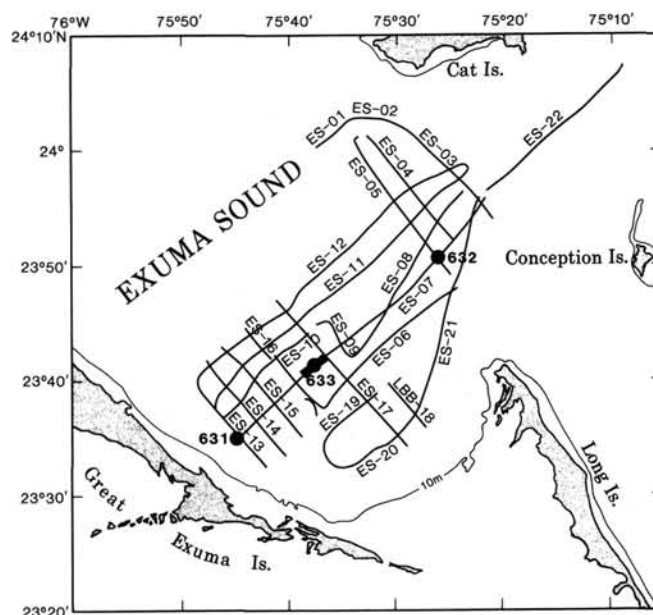
Figure 15. Site-survey grid in southeastern Exuma Sound. Navigation was accomplished by integrating LORAN C, Transit satellite, and radar bearings off nearby islands. Locations of Sites 631, 632, and 633 are shown (see Austin, Schlager, et al., 1986). The portion of ES-07 shown in Figure 17 is indicated by the bold line. All profiles are 24-trace, 12-fold, collected with a 400-in. 3 water gun (see also Austin et al., this volume).
