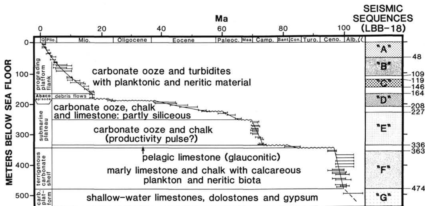
Figure 8. Geologic history of Site 627 (see also Austin, Schlager, et al., 1986). Accumulation-rate curve includes biostratigraphic age control (horizontal bars) and hiatuses (horizontal wavy lines). Seismic stratigraphy at the site is along the right-hand margin (refer also to Fig. 7), and the genetic interpretation of the sampled sediments on the left-hand margin. The F/G sequence boundary correlates in depth with the top of the upper Albian shallow-water carbonate platform.
