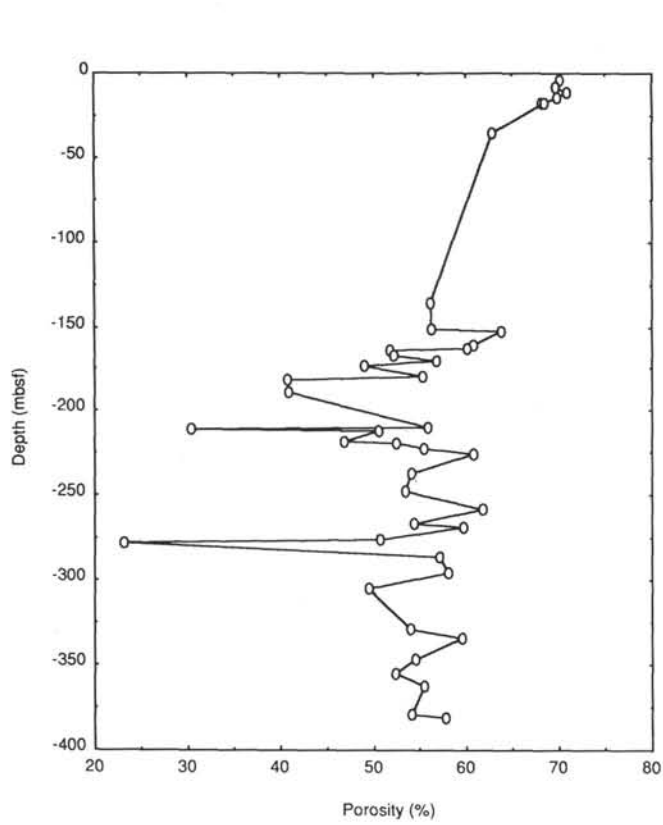
Figure 14. Porosity profile for Site 694.
