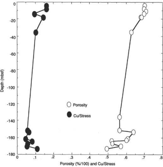
Figure 15. Ratio of undrained shear strength to vertical effective stress and porosity plotted against depth for Site 694. Ratios between 0.2 and 0.5 are considered normally consolidated.
