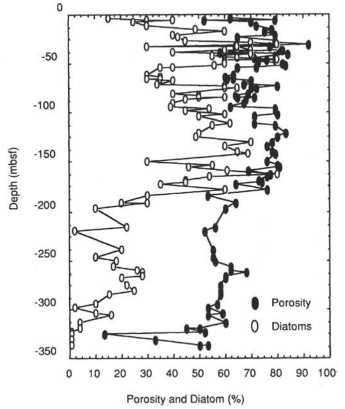
Figure 16. Profiles of porosity and percent diatoms vs. depth for Site 695A.
