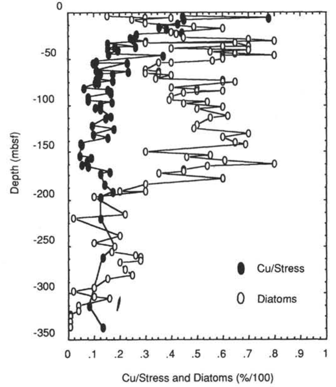
Figure 17. Ratio of undrained shear strength to vertical effective stress and decimal percent diatoms for Hole 695A, plotted against depth.
