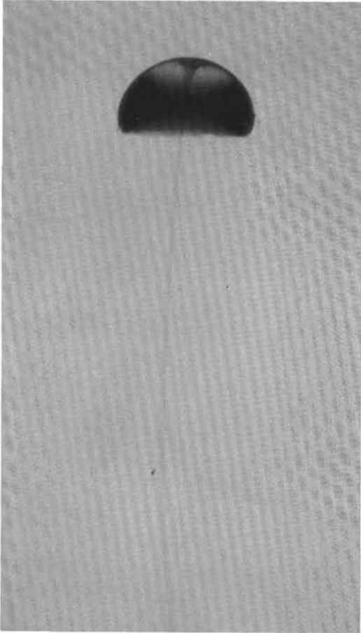
A. Photograph of a plume formed by injection of a warm glucose solution (colored with dye) into the base of a large tank of cooler, clear glucose. The Réunion mantle plume may have formed such a diapiric structure: the large spherical head would have melted to produce the Deccan flood basalt event at 66 Ma, whereas the narrow tail supplied the subsequent hotspot track. (Photo by R. Griffiths.) B. The Western Ghats, a 2-km-thick section of the Deccan flood basalts. The estimated original volume of basaltic magma ( >1.5 \times 10^6 \text{ km}^3 ) was erupted in less than 1 m.y. at the beginning of Réunion hotspot activity. (Photo by J. Mahoney.)
