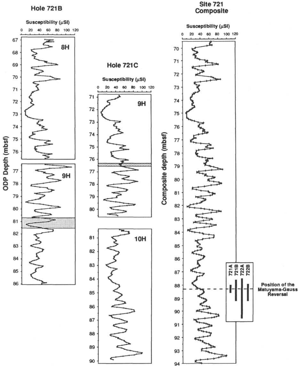
Figure 3. Interhole correlations using the magnetic susceptibility data. The shaded areas represent the missing section between core breaks; these were used to construct a complete composite sequence, a portion of which is shown to the right of the figure. The susceptibility data were also used to constrain the position of the Matuyama-Gauss Chronozone boundary (2.47 Ma; 88.30 mbsf composite depth) based on data from Holes 721A, 721B, 722A, and 722B.
