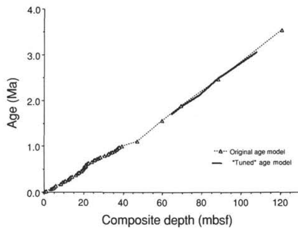
Figure 11. Comparison of the preliminary age model of Figure 8 with the "tuned" age model shown in Figure 10.
