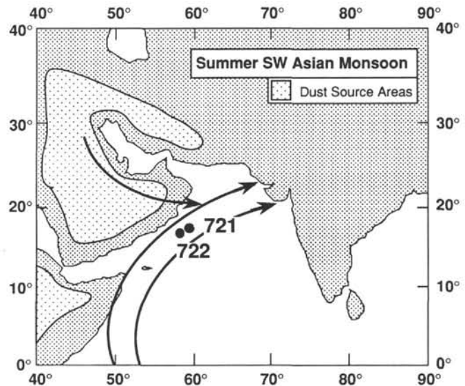
Figure 1. Lower tropospheric (1–2 km altitude) wind fields over the Arabian Sea during the summer monsoon (after Hastenrath and Lamb, 1980). Eolian dust source areas are based on satellite imagery from Sirocko and Sarnthein (1989).
