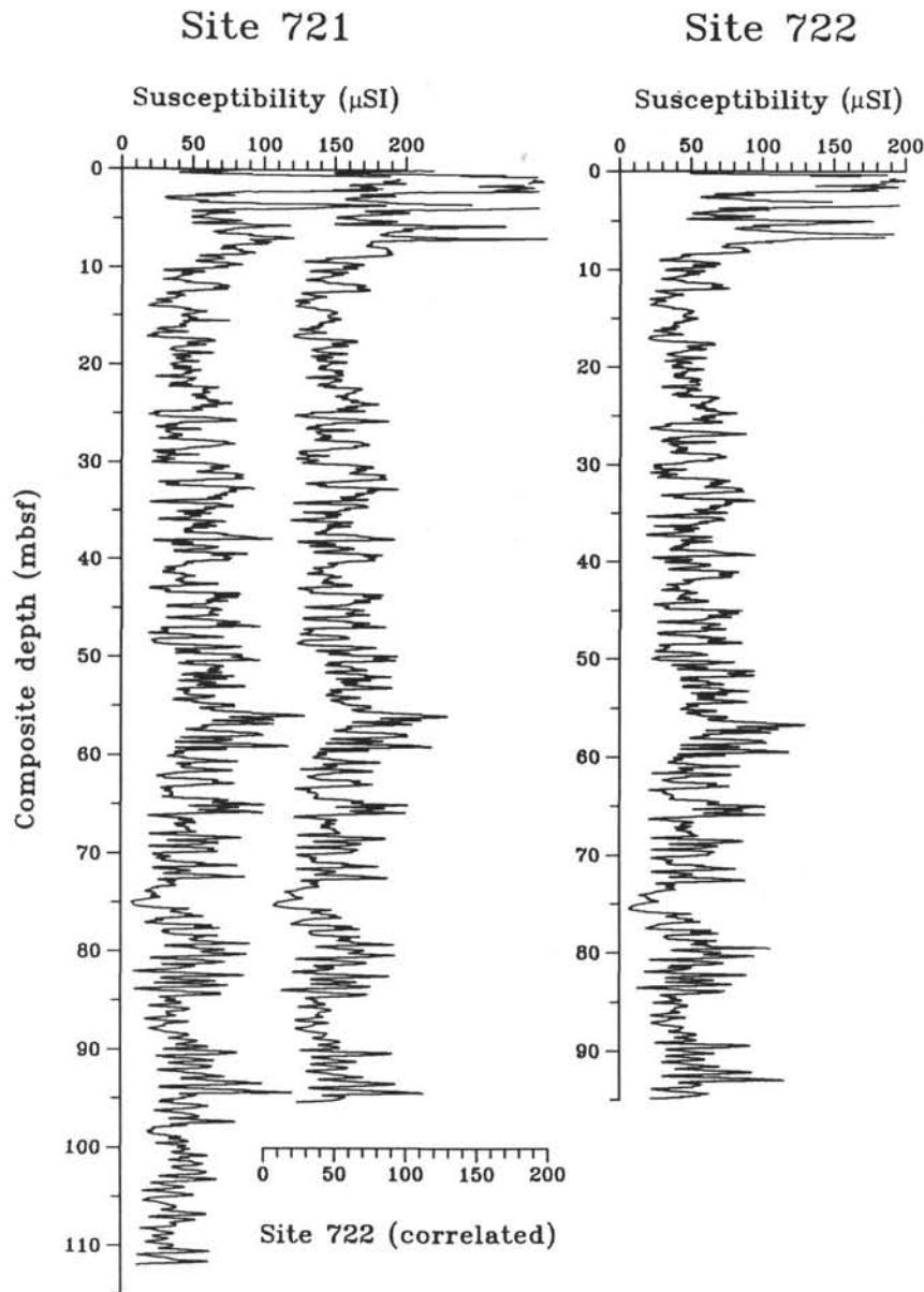
Figure 4. Depth plots of the composite magnetic susceptibility records from Sites 721 and 722. The middle curve is the Site 722 susceptibility record correlated to the Site 721 record using the inverse correlation program of Martinson et al. (1984). The coherence between the correlated Site 722 data and Site 721 is high (0.95).
