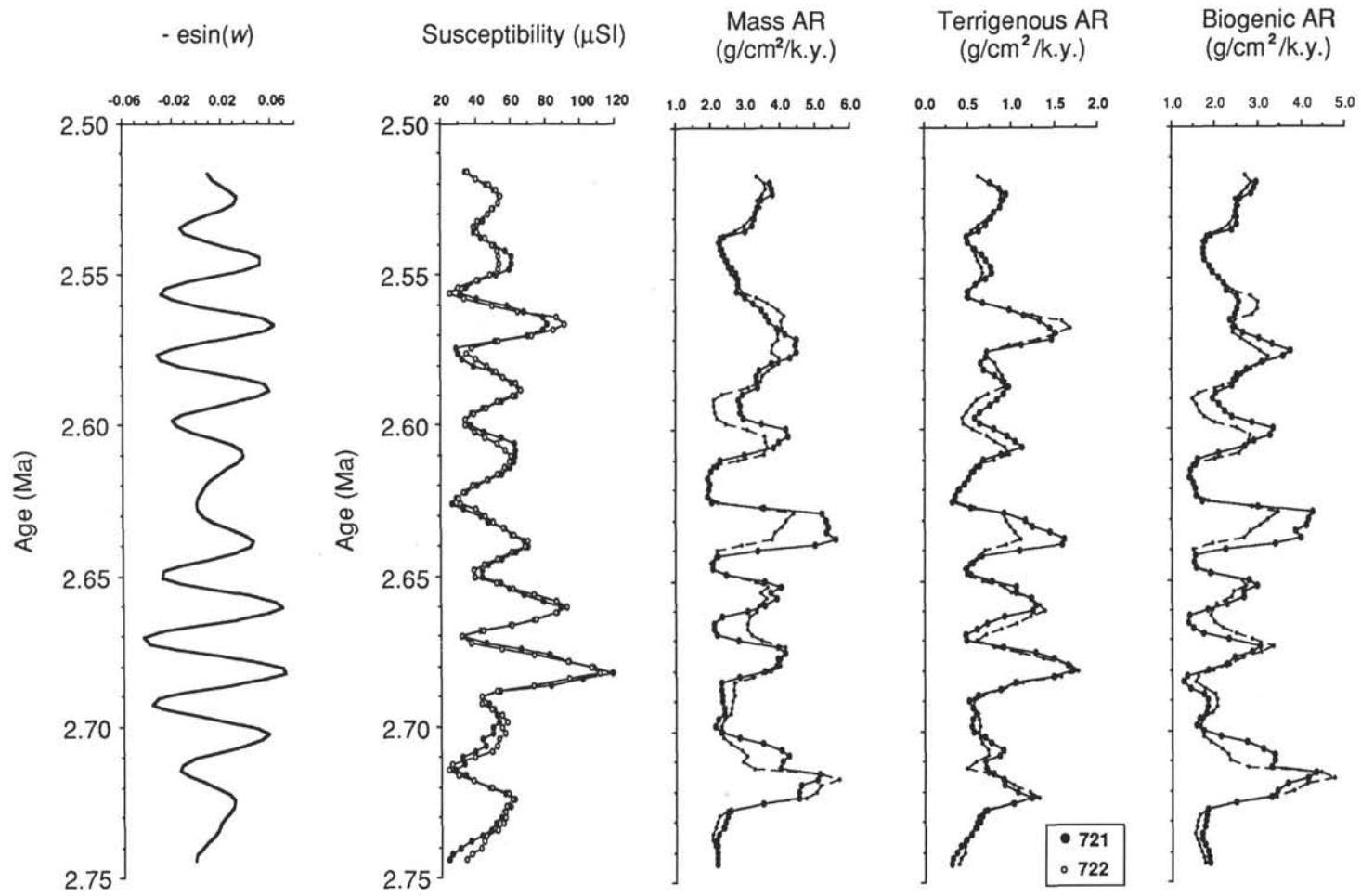
Figure 14. Terrigenous and biogenic component flux calculations based on the "tuned" time scale (2.75–2.55 Ma). Susceptibility data from Sites 721 and 722 were correlated to orbital precession and variations in sedimentation rate were calculated and used to determine downcore mass accumulation rates. The similar data between sites suggests that the results are real and not site-dependent. Terrigenous and biogenic accumulation rates were calculated using the terrigenous-susceptibility regression equation shown in Figure 6.
