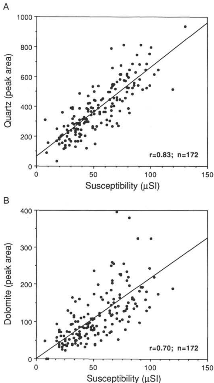
Figure 5. Correlations of bulk X-ray diffraction estimates of quartz (A) and dolomite (B) abundances with magnetic susceptibility. Previous aerosol and sediment studies have identified an eolian origin for these minerals in the Arabian Sea (Stewart et al., 1965; Goldberg and Griffin, 1970; Sirocko and Sarin, 1989).
