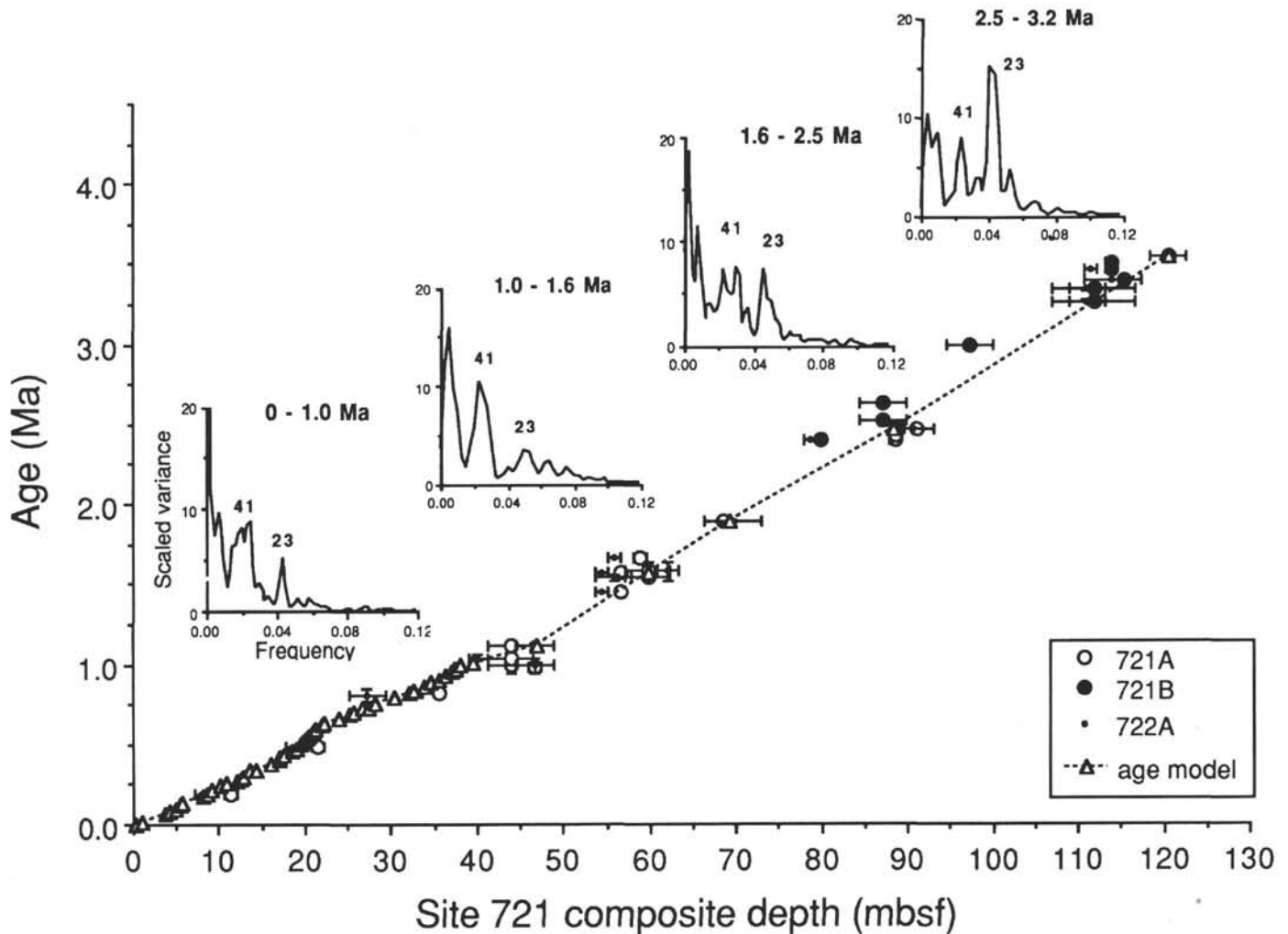
Figure 7. Age-depth relations for the Site 721 composite sequence. Age datums from Holes 721A, 721B, and 722A were transferred to their appropriate depths in the Site 721 composite sequence so that a maximum number of datums (46) could be used to determine the preliminary age model shown by the triangles and dotted line. Oxygen isotope data were used to determine age-depth relations to 1.0 Ma (Clemens and Prell, this volume); these datums are listed in Table 2. Power spectra of the susceptibility data were calculated for four separate intervals: 0–1.0 Ma, 1.0–1.6 Ma, 1.6–2.5 Ma, and 2.5–3.2 Ma (bandwidth = 0.004). Note that the data vary predominantly at orbital periodicities, and that these periodicities are nonstationary over the 3.2 Ma record.
