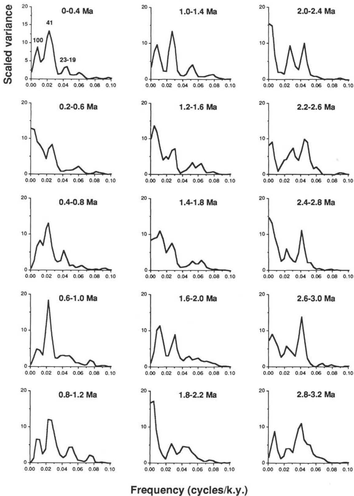
Figure 12. Power spectra calculated for overlapping 400 k.y. segments of the susceptibility time series. Note that the first increase in 41 k.y. power occurs in the 2.2-2.6 Ma window and is fully represented in the 2.0-2.4 Ma window, indicating that the shift takes place at ~2.4 Ma.
