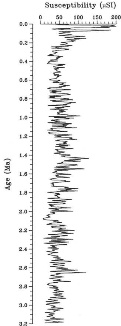
Figure 8. The magnetic susceptibility time-series based on the age model shown in Figure 7.
