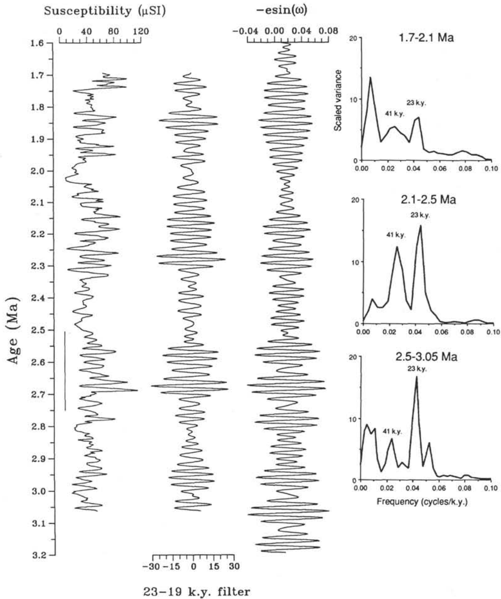
Figure 10. Calculated precession ( -\text{esin}(\omega) ), the 23-19 k.y. band-pass filter of the susceptibility record, and the raw susceptibility record for the 3.2-1.6 Ma interval. The filtered susceptibility data were correlated (phase-locked) to precession using a signal correlation package (Martinson et al., 1984) to investigate the degree of coherency between the presumed isolation forcing ( -\text{esin}(\omega) ) and the climate response (susceptibility). The coherency is particularly high (0.89) between precession and the filtered susceptibility over the 3.2-2.5 Ma interval, the coherency of the entire 3.2-1.6 Ma interval is 0.86. Power spectra are shown for three intervals (3.2-2.5 Ma, 2.5-2.1 Ma, and 2.1-1.6 Ma) to demonstrate the increase in 41 k.y. power after 2.5 Ma (bandwidth = 0.004). The vertical line to the left shows the interval selected for the flux calculations described in the text and shown by Figures 13-15.
