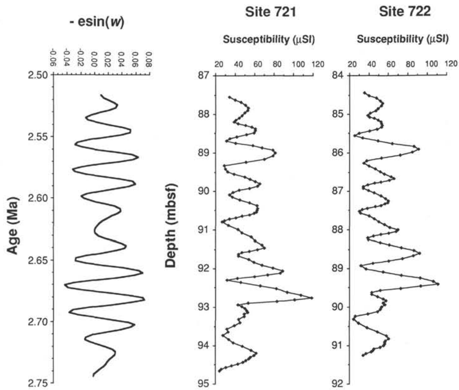
Figure 13. Calculated precession ( -\text{esin}(\omega) ) for 2.75–2.55 Ma and the raw susceptibility data from the Site 721 and 722 composite records that correspond to this time interval.
