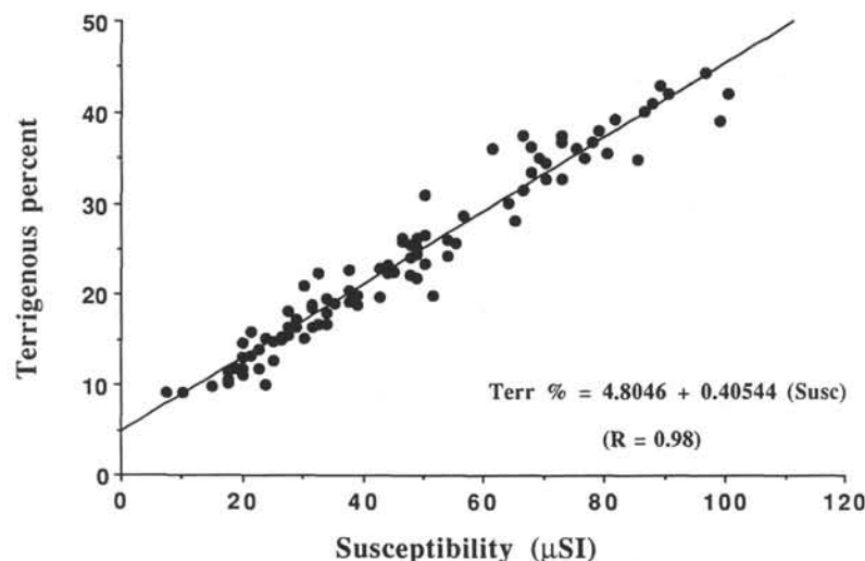
Figure 6. Correlation between terrigenous percent (determined after the sequential extraction of carbonate, opal, and organic carbon) and magnetic susceptibility. The extremely high correlation suggests that susceptibility can be used as a rapid and conservative tracer of the terrigenous fraction variations. The negative x-intercept value indicates that there is no background supply of magnetic material unassociated with the terrigenous fraction.
