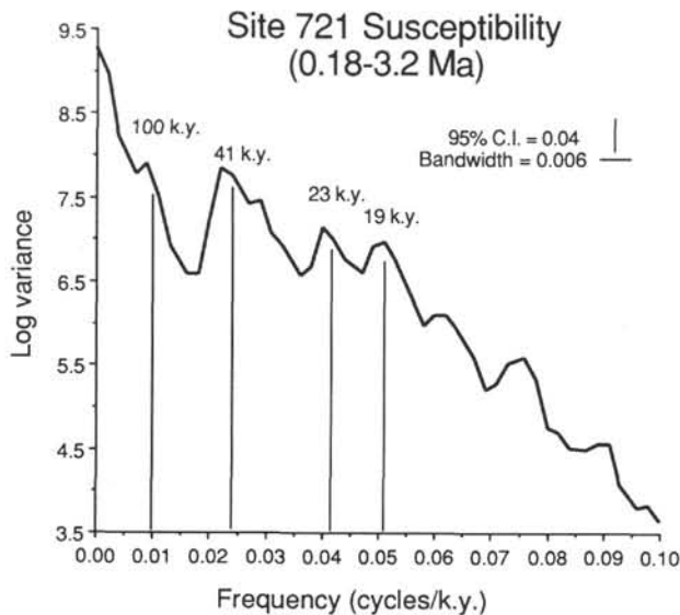
Figure 9. Power spectral estimates of the susceptibility time-series shown in Figure 8 (the uppermost 180 k.y. of the record was excluded). Note that much of the variance is centered at orbital periodicities.
