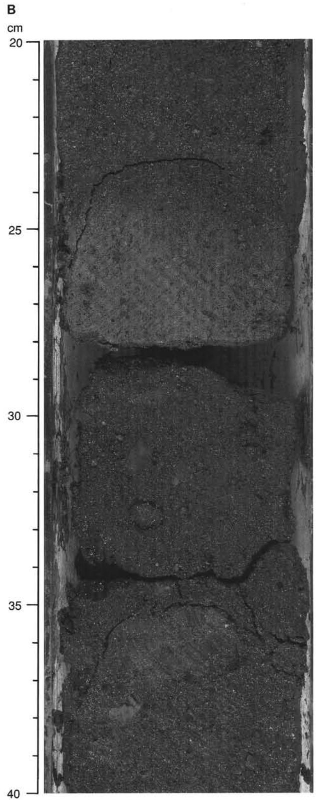
A. Laminated calcareous claystone, 15 cm-thick, at the Cretaceous/Tertiary boundary in Section 738C-20R-5 from the southern Kerguelen Plateau. Arrow points to 2-mm-thick clay layer enriched in iridium. B. Massive diamictite of early Oligocene age from Section 739C-40R-1 from the Prydz Bay continental shelf. These and other glacial sediments recovered in Prydz Bay are evidence of extensive Antarctic glaciation in early Oligocene, and possibly late Eocene, time.
