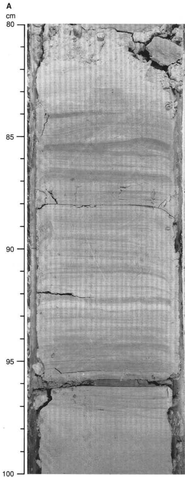
A. Laminated calcareous claystone, 15 cm-thick, at the Cretaceous/Tertiary boundary in Section 738C-20R-5 from the southern Kerguelen Plateau. Arrow points to 2-mm-thick clay layer enriched in iridium. B. Massive diamictite of early Oligocene age from Section 739C-40R-1 from the Prydz Bay continental shelf. These and other glacial sediments recovered in Prydz Bay are evidence of extensive Antarctic glaciation in early Oligocene, and possibly late Eocene, time.
