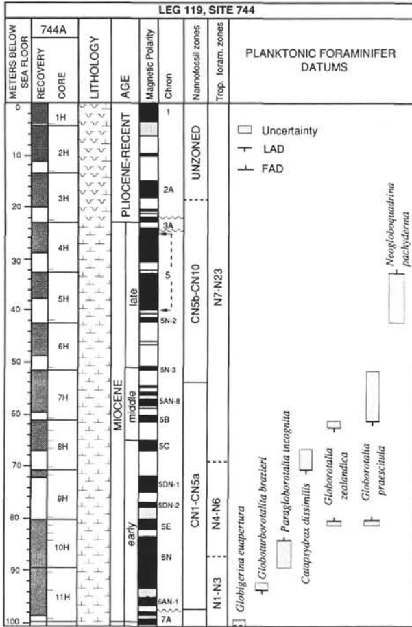
Figure 4. Lithostratigraphy and biostratigraphy of the uppermost Eocene through Holocene sequence recovered at ODP Site 744 based on biostratigraphic data presented in Table 3. See Figures 2 and 3 for additional explanation.
