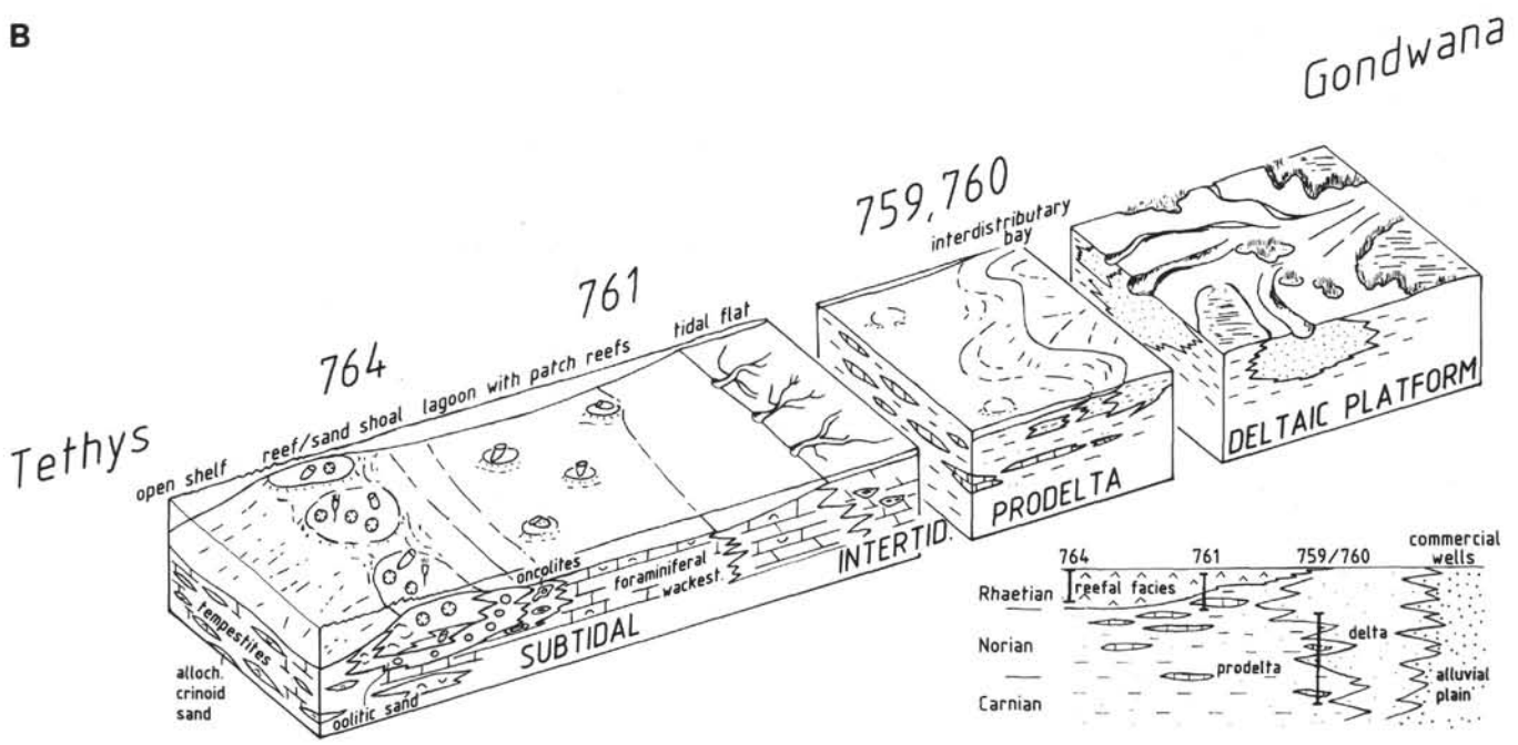
A. Schematic east-west and north-south sections across the Exmouth Plateau and adjacent abyssal plains with approximate locations of ODP sites. Note the marked post-rift unconformity underlain by block-faulted Triassic (-Jurassic) sediments and overlain by a thin cover of post-breakup sediments (modified from Exon et al., this volume, chapter 1). B. Generalized facies model for the Wombat Plateau Upper Triassic (northeast Gondwanan margin). Sites 759 and 760 represent the fluviodeltaic-dominated series of the Carnian and Norian, and Sites 761 and 764 represent the Rhaetian carbonate platform (Site 761: intertidal to shallow subtidal lagoon; Site 764: subtidal oolite shoals, reefs, and reefal debris) (from Röhl et al., this volume, chapter 7).
