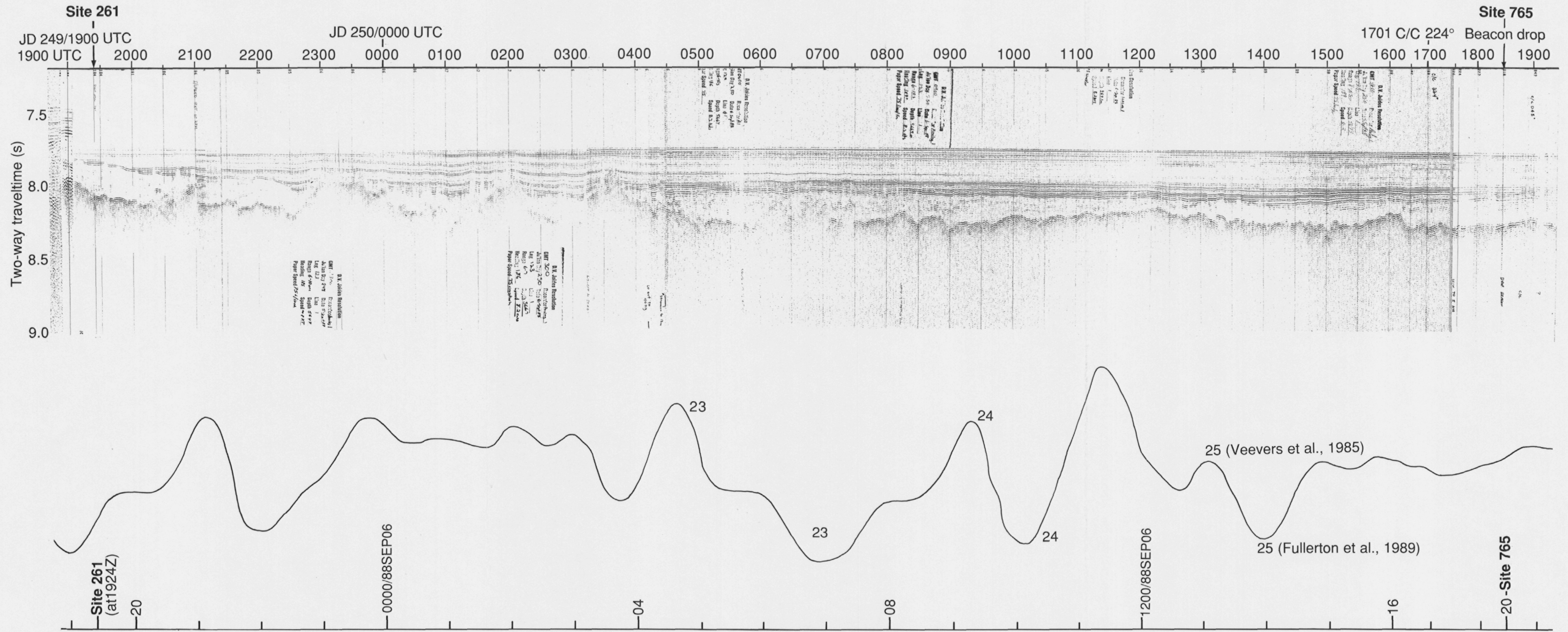
Volume 123: Chapter 2: Figure 9. Shipboard monitor records of seismic Line 1 shot between Sites 261 and 765. Below is a profile of corrected magnetic data showing best correlation with marine magnetic anomalies M23 through M25, postulated for the Argo Abyssal Plain by Veevers et al. (1985) and Fullerton et al. (1989).
