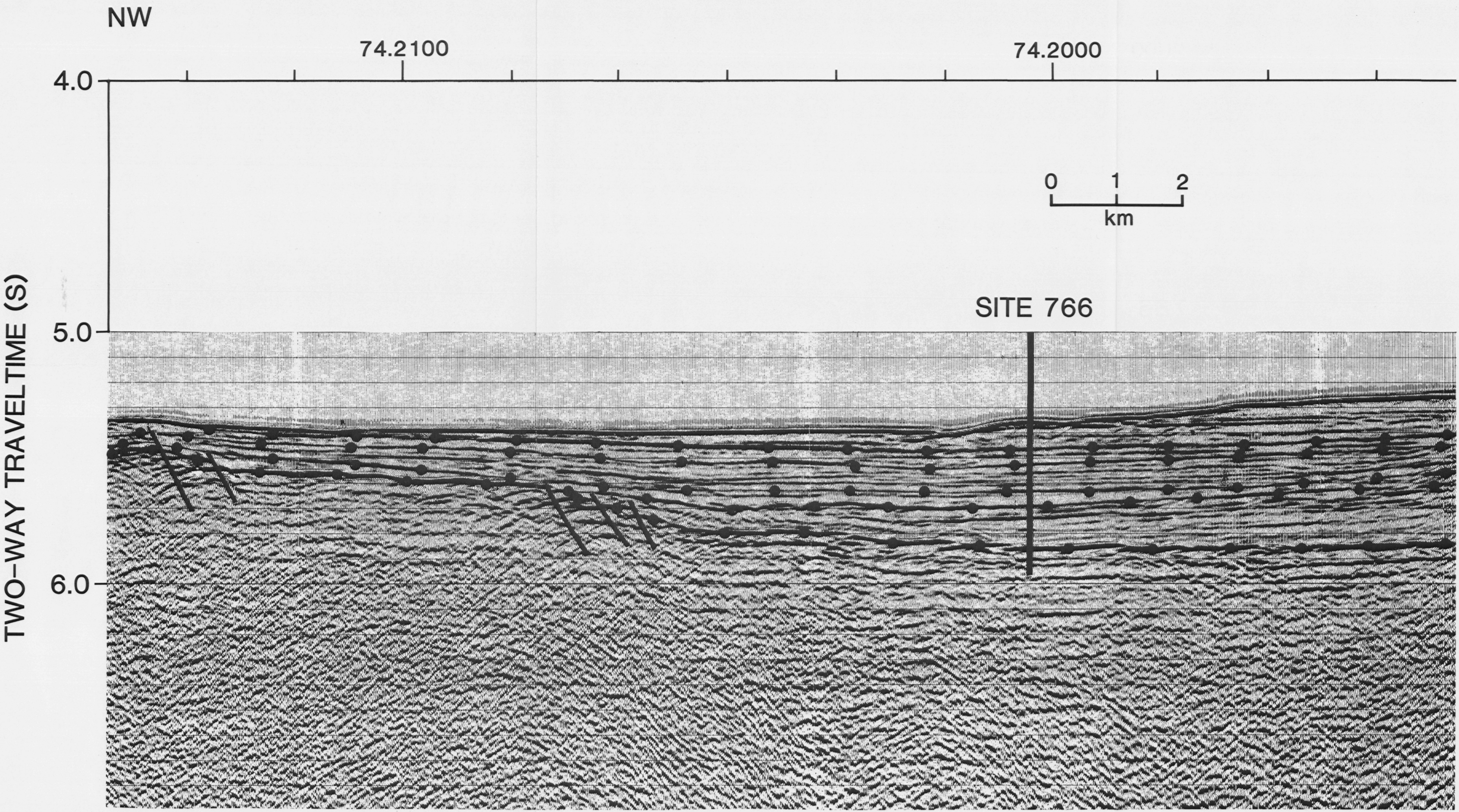
Volume 123: Chapter 31: Figure 12. BMR multifield seismic Line 55/2 showing distribution and seismic character of sequences across entire study area. See Figure 3 for location.
