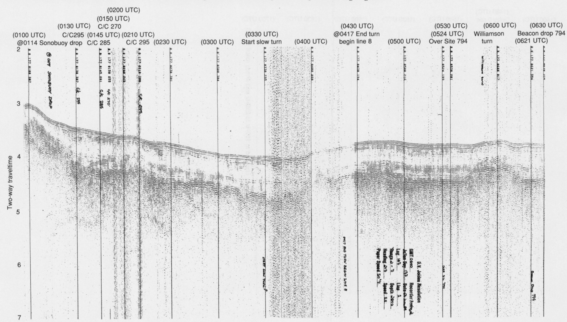
Volume 127A: Chapter 3: Figure 4. All unprocessed single-channel seismic profiles acquired during Leg 127.
