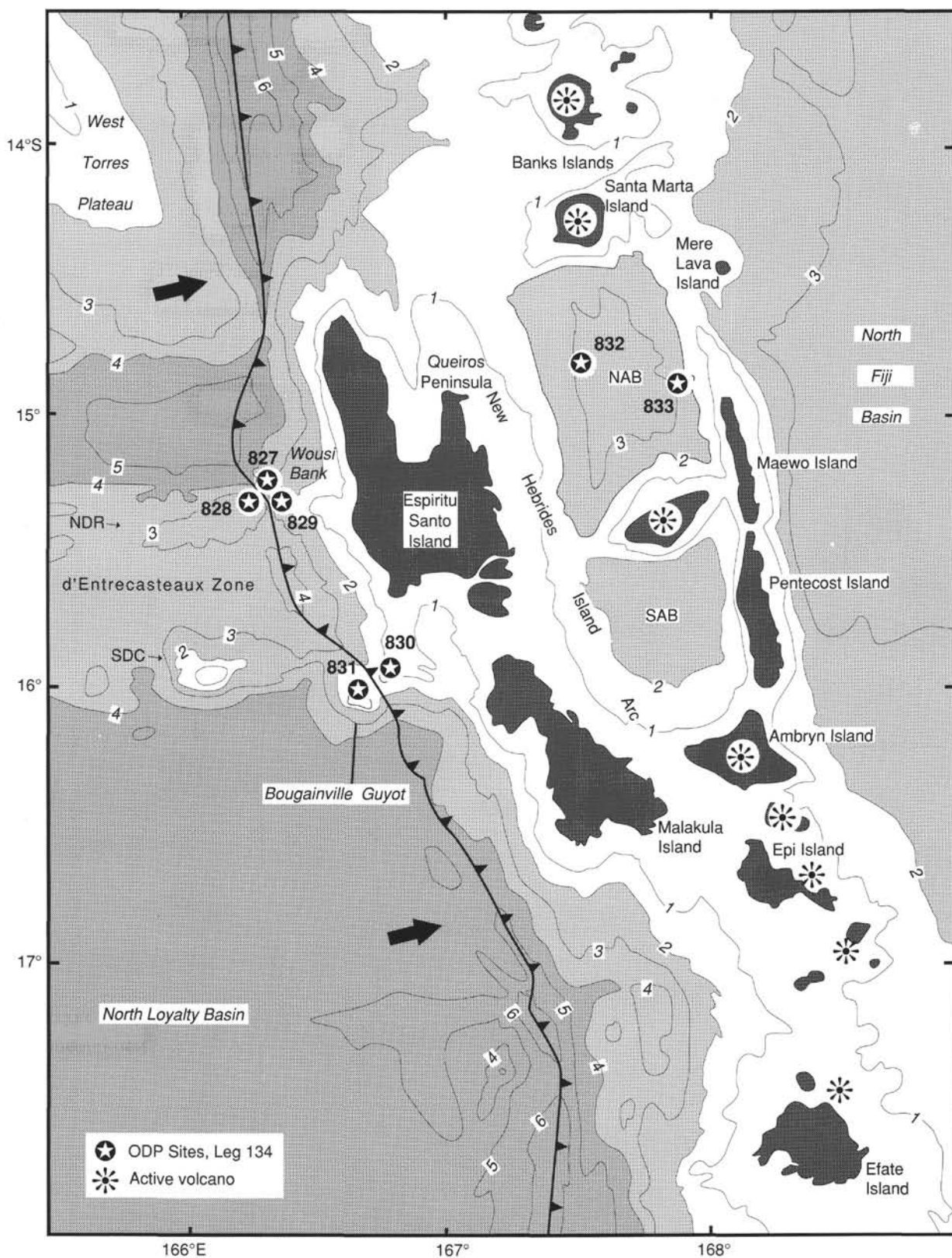
Location of Leg 134, Sites 827–833, central New Hebrides Island Arc. Bathymetry in kilometers. NDR = North d'Entrecasteaux Ridge, SDC = South d'Entrecasteaux Chain, NAB = North Aoba Basin, SAB = South Aoba Basin. Bold line with teeth indicates approximate position of subduction zone; teeth are on upper plate. Arrows indicate direction of plate convergence.
