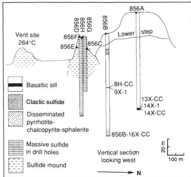
Figure 3. South-north cross section of Site 856 showing drilled holes and the massive sulfide mound. Vertical scale is at x5 exaggeration.
