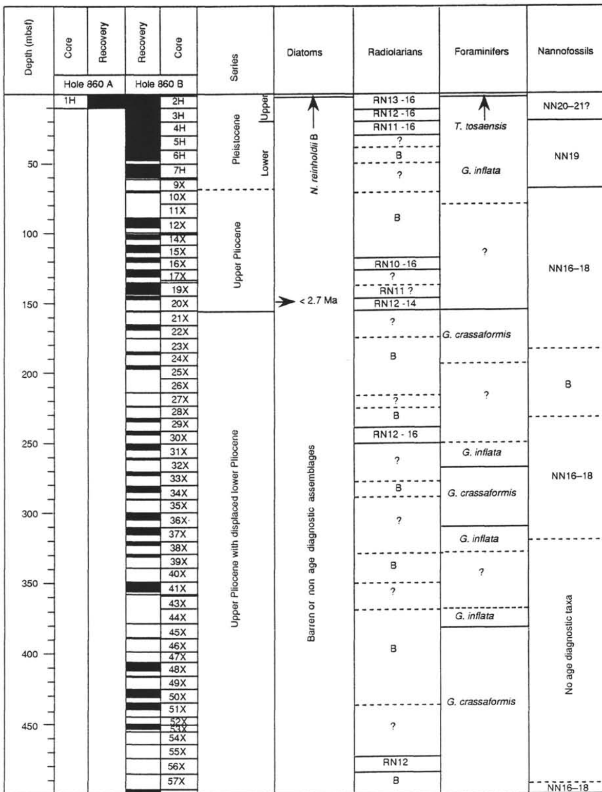
Figure 15. Summary of biostratigraphic age for the sediments recovered at Site 860. B = barren.
