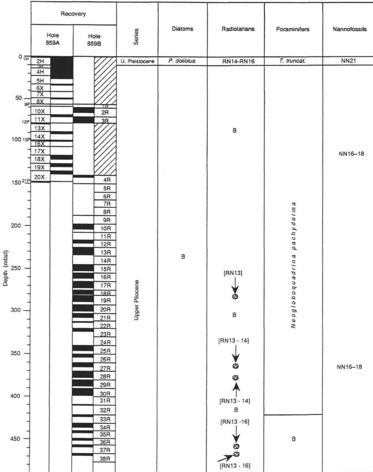
Figure 12. Summary of biostratigraphic age for the sediments recovered at Site 859. B = barren.
