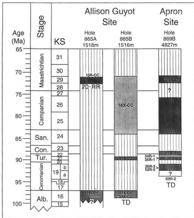
Figure 3. Age of Cenomanian to Maastrichtian sediments, dated by planktonic foraminifers from Leg 143. Albian shallow-water limestone shown by lithologic symbol, dated primarily by benthic foraminifers (Arnaud-Vanneau and Sliter, this volume). Zone assignment as in Figure 2. Dark stipple = dated to zone; light stipple = poorly dated interval. TD = total depth.
