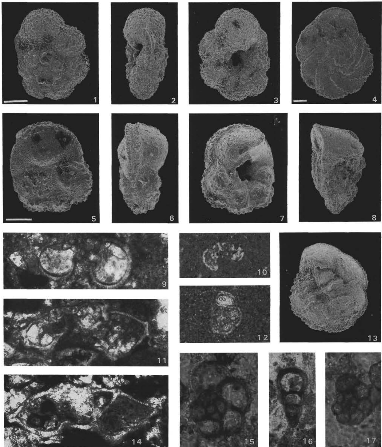
Plate 3. Scale bar = 100 \mu m. 1-3. Whiteinella aprica (Loeblich and Tappan), spiral, side and umbilical views, Sample 143-865B-17X-CC, 14-16 cm. 4, 8, 13. Globotruncanita elevata (Brotzen), spiral, side and umbilical views, Sample 143-869B-12R-CC. 5-7. Globotruncana aegyptiaca (Nakkady), spiral, side and umbilical views, Sample 143-869B-10R-CC. 9. Whiteinella baltica (Douglas and Rankin), axial section, Sample 143-869B-34R-1, 142-144 cm, 150 \times . 10. Hedbergella sp. cf. H. trocoidea (Gandolfi), transverse section, Sample 143-865A-79R-1, 32-33 cm, 300 \times . 11. Dicarinella imbricata (Mornod), axial section, Sample 143-869B-35R-1, 44-46 cm, 150 \times . 12. Ticinella? sp. cf. T. primula (Luterbacher), transverse section, Sample 143-866A-36R-1, 2-4 cm, 300 \times . 14. Rotalipora sp. cf. R. greenhornensis (Morrow), oblique axial section, Sample 143-969B-52R-5, 12-15 cm, 150 \times . 15. Hedbergella monmouthensis (Olsson), transverse section, Sample 143-869B-30R-1, 24-26 cm, 300 \times . 16. Heterohelix reussi (Cushman), edge section, Sample 143-869B-30R-1, 24-26 cm, 300 \times . 17. Hedbergella planispira (Tappan), transverse section, Sample 143-869B-30R-1, 24-26 cm, 150 \times .
