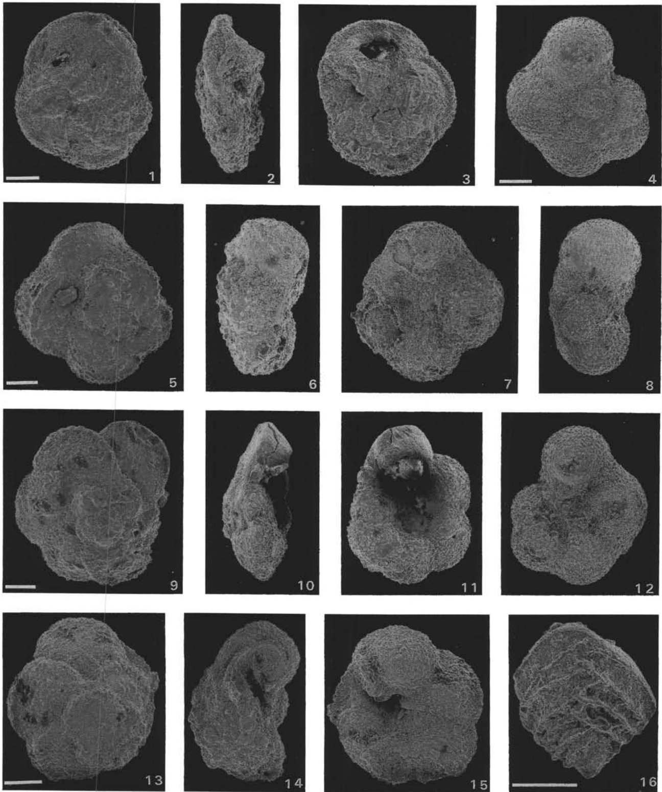
Plate 2. Scale bar = 100 \mu m. 1–3. Dicarinella primitiva (Dalbiez), spiral side and umbilical views, Sample 143-869B-31R-1, 72–74 cm. 4, 8, 12. Whiteinella baltica (Douglas and Rankin), spiral, side and umbilical views, Sample 143-869B-31R-1, 72–74 cm. 5–7. Helvetoglobotruncana helvetica (Bolli), spiral, side and umbilical views, Sample 143-865B-17X-CC, 14–16 cm. 9–11. Marginotruncana sigali (Reichel), spiral, side and umbilical views, Sample 143-869B-31R-1, 72–74 cm. 13–15. Praeglobotruncana gibba (Klaus), spiral, side and umbilical views, Sample 143-865B-17X-CC, 14–16 cm. 16. Aragonia ouezzaensis (Rey), side view, Sample 143-869B-11R-CC.
