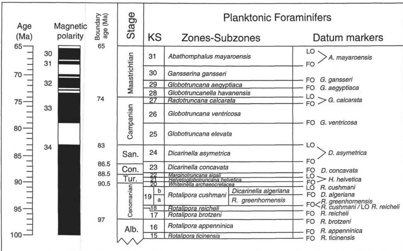
Figure 2. Zonation for Cretaceous planktonic foraminifers examined in thin section (after Sliter, 1989; modified from Caron, 1985). Magneto-geochronology after Harland et al. (1990). KS = Cretaceous zone notation; FO = first occurrence; and LO = last occurrence.
