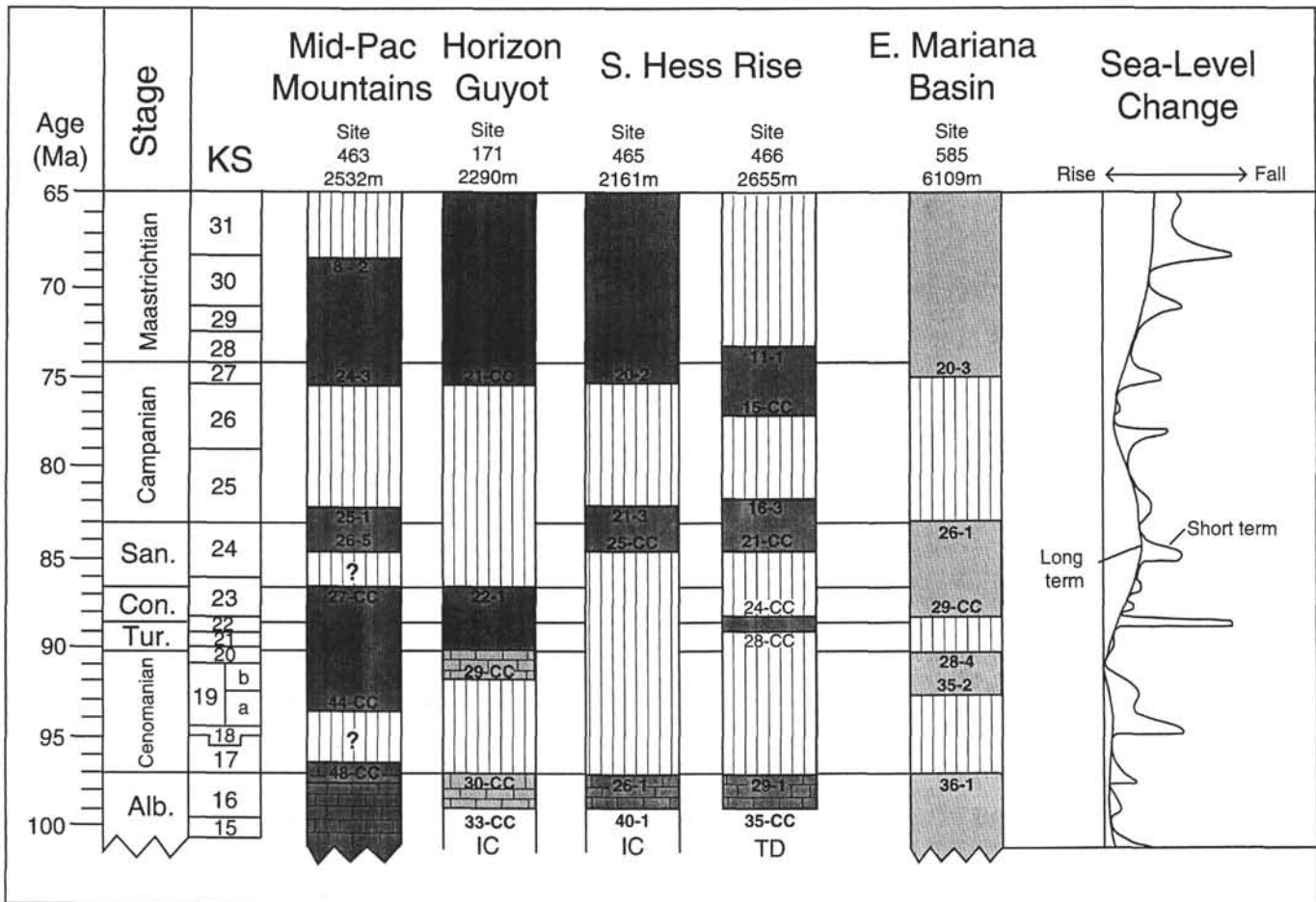
Figure 5. Age of Cretaceous sediments dated by planktonic foraminifers from selected DSDP sites in the central Pacific Ocean and East Mariana basins. Zone assignments as in Figure 2. Patterns and abbreviations as in Figure 3. Lithologic symbols shown for chalk and limestone. IC = igneous crust. Sea-level curve modified from Haq et al. (1987).
