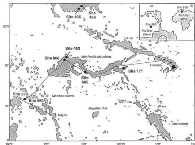
Figure 1. Location of Leg 143 drill sites and nearby DSDP sites that contain Cretaceous planktonic foraminifers (black circles). Shaded areas are shallower than 4 km. Line shows track of JOIDES Resolution . Inset: Location of DSDP Site 585 in the East Mariana Basin. Shaded areas are shallower than 5 km.
