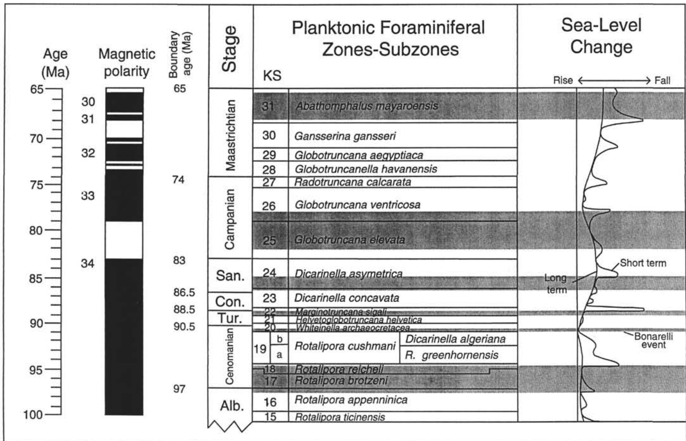
Figure 6. Stratigraphic distribution of hiatuses in Late Cretaceous pelagic cover at DSDP sites in the central Pacific Ocean Basin relative to changes in sea level. Hiatuses = shaded areas. Sea-level curve modified from Haq et al. (1987).
