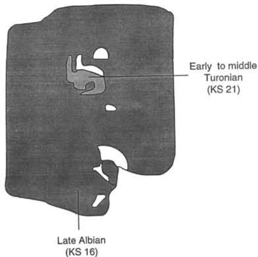
Figure 4. Sketch of core sample of late Albian shallow-water limestone from Section 143-865B-17X-CC showing several solution cavities (open areas) and location of early to middle Turonian cavity fill (light stipple) containing planktonic foraminifers.
