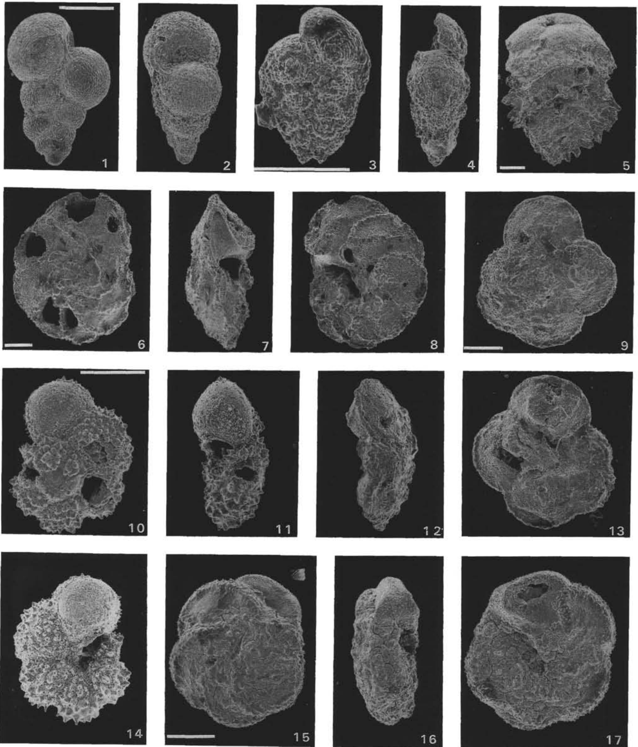
Plate 1. Scale bar = 100 \mu m. 1, 2. Heterohelix reussi (Cushman), side and edge views, Sample 143-865B-17H-CC, 14–16 cm. 3, 4. Heterohelix carinata (Cushman), side and edge views, Sample 143-869B-28R-CC. 5. Reussella szajnochae (Grzybowski), side view, Sample 143-869B-15R-CC. 6–8. Rotalipora greenhornensis (Morrow), spiral, side and umbilical views, Sample 143-869B-36R-13, 13–14 cm. 9, 12–13. Rotalipora cushmani (Morrow), spiral, side and umbilical views, Sample 869B-31R-1, 72–74 cm. 10, 11, 14. Dicarinella algeriana (Caron), spiral, side and umbilical views, Sample 143-869B-44R-1, 127–128 cm. 15–17. Dicarinella canaliculata (Reuss), spiral, side and umbilical views, Sample 143-869B-31R-1, 72–74 cm.
