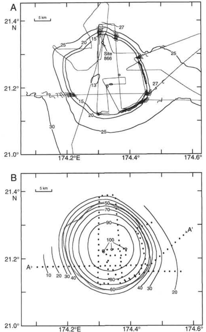
Figure 2. Bathymetry (A) and free-air gravity anomaly (B) maps of Resolution Guyot. Bathymetry contours are shown at 500-m intervals, except where SeaBeam multibeam echo-sounder contours are shown at 100-m intervals. Bathymetry contours are labeled in hundreds of meters. Light gray lines show ship tracks. Gravity contours are shown at 10-mGal intervals and are labeled in mGals. A heavy gray contour shows the 2000-m bathymetry contour for reference. Dots show location of gravity data points used for modeling; "A" and "A'" show the beginning and end points of the profile shown in Figures 8 and 9.
