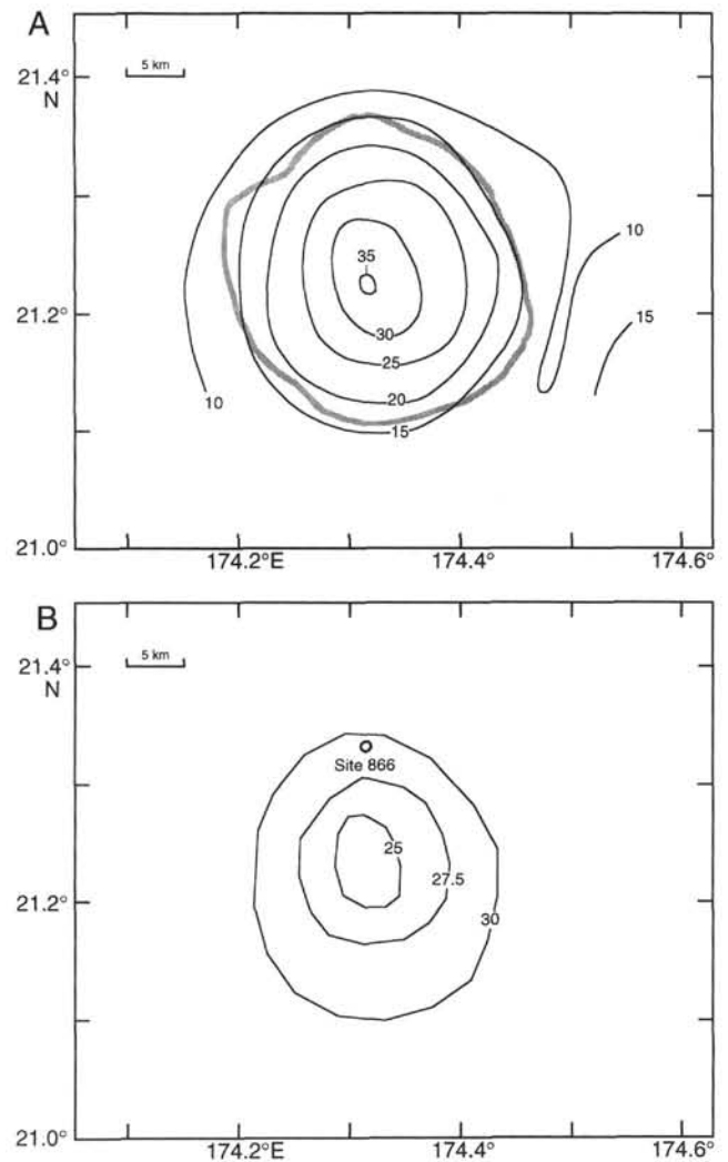
Figure 6. Resolution Guyot residual gravity anomaly (A) and residual mass anomaly model (B) for the residual gravity anomaly. The residual anomaly was determined by subtracting the calculated gravity anomaly (Fig. 5) from the observed anomaly (Fig. 2). Anomaly contours are shown at 5-mGal intervals and labeled in mGal. Heavy gray contour shows the 2000-m bathymetry contour. Polygons in B represent the vertical edges of prisms used for the gravity model calculations (Plouff, 1976). Contours are labeled by depths used in Model C6 (Table 1). Location of Site 866 shown by open circle.
