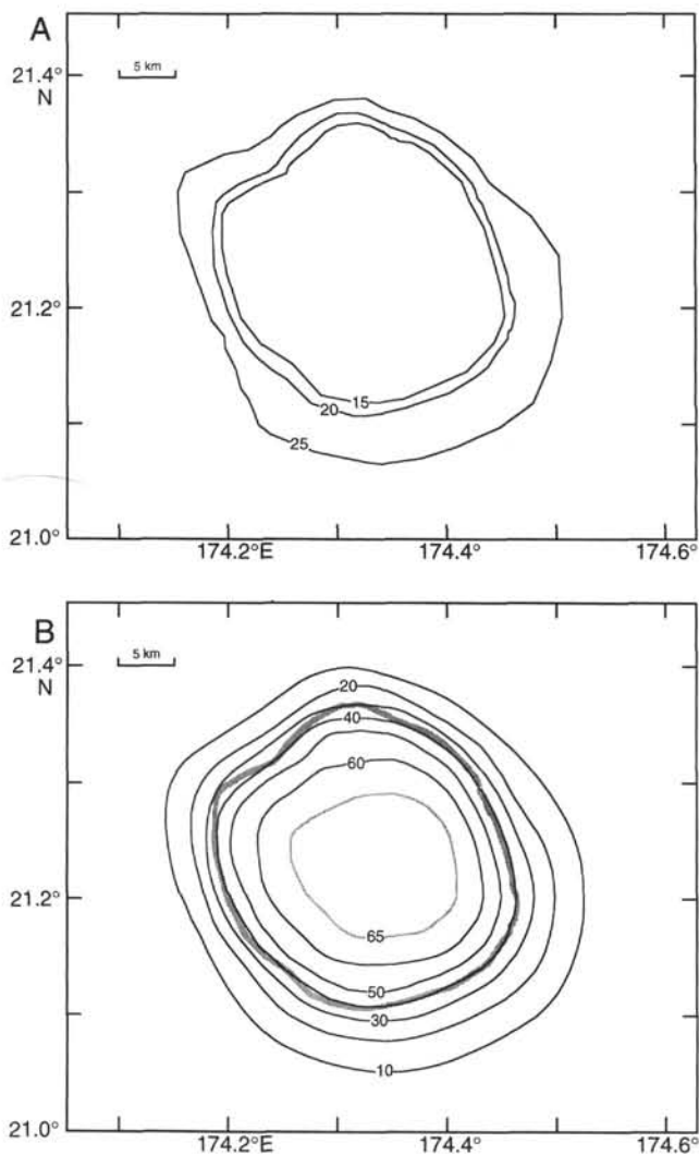
Figure 5. Bathymetry model (A) and calculated free-air anomaly (B) of Resolution Guyot. Lines on the model map represent the vertical sides of polygonal prisms used to represent the bathymetry (Plouff, 1976). These are labeled by the depths of the bathymetry contours (in hundreds of meters) used to constrain their shape. Calculated free-air anomaly contours are shown at 10-mGal levels, except for the 65 mGal contour, which is shown in gray. The heavy gray contour shows the 2000-m bathymetry contour.
