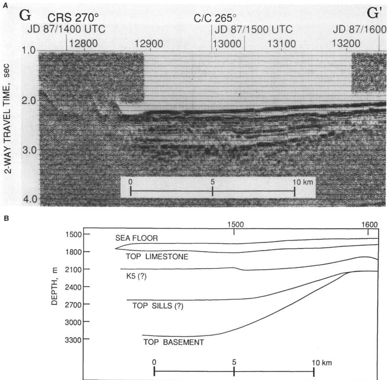
Figure 17. Profile across southeastern part of Allison Guyot. Location shown by Line G-G' in Figure 3. A. Processed (0.2 s AGC, mixed) seismic line, showing buried volcanic basement topography. Reflector at 2.90 s two-way traveltime is interpreted as corresponding to the sills drilled at Site 865. The limestone strata onlap the basement progressively to the west (right). Vertical exaggeration at the seafloor is about 4 \times . B. Depth section along the line of the seismic profile, using the velocity structure determined from drilling at Site 865, extrapolated to basement using an average velocity of 3.3 km/s in the limestones between the sills and basement (from Winterer et al., this volume).
