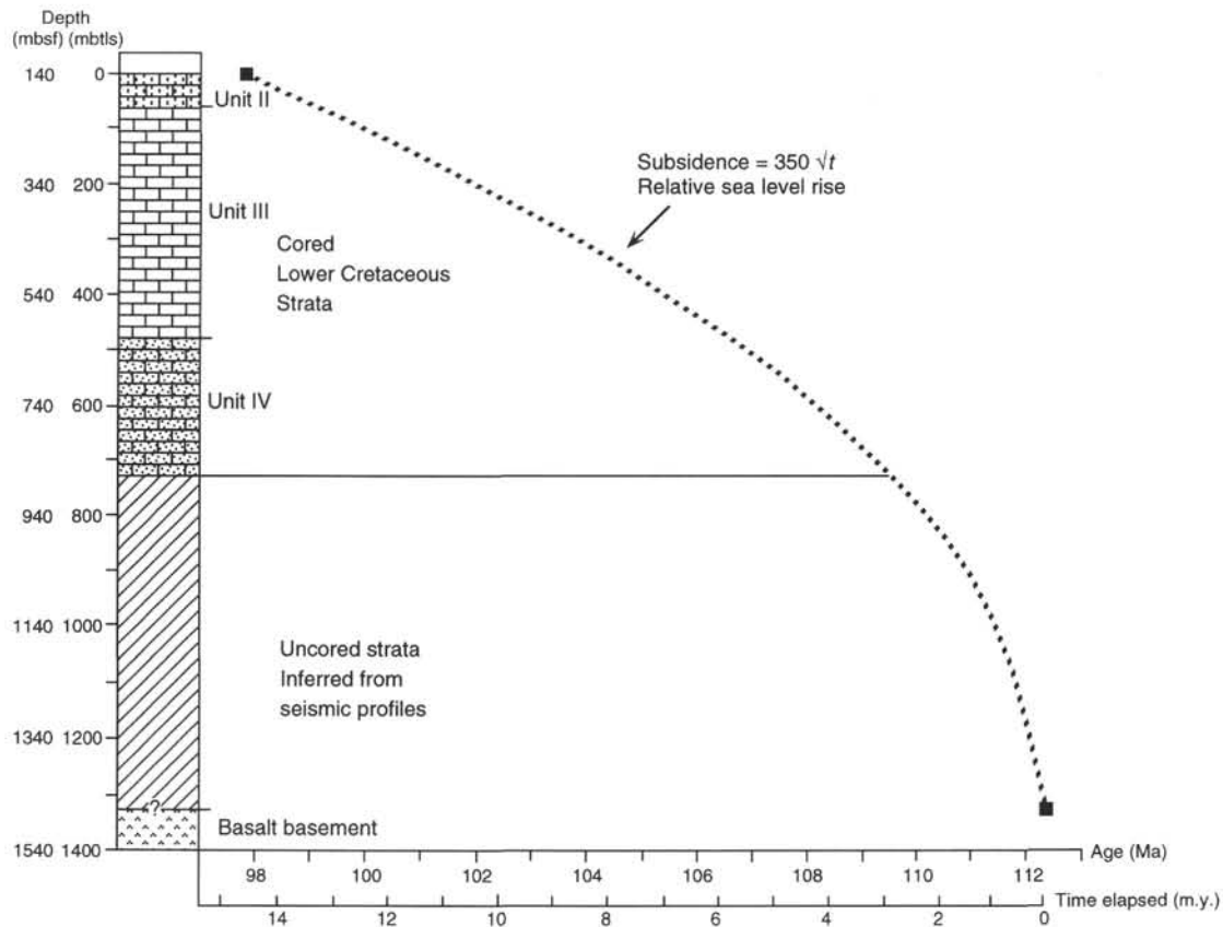
Figure 18. Inferred subsidence curve for Site 865 on Allison Guyot. The curve was constructed using an age of 98 Ma for the top of the limestone section, and a total thickness of 1330 m for the limestone, consisting of the actual drilled thickness at Hole 865A, plus the additional, undrilled thickness estimated from the seismic profile (Fig. 17).
