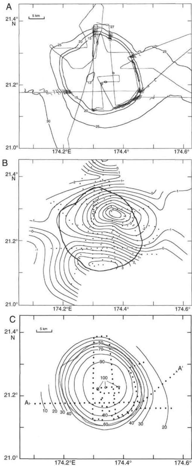
Figure 24. Bathymetry (A), magnetic anomaly (B), and gravity anomaly (C) over Resolution Guyot. Bathymetric contours at 100-m intervals where multibeam echo-sounder data are available. Heavy contours are at 500-m intervals, labeled in hundreds of meters. Magnetic anomaly contours are at 50-nT intervals, labeled in hundreds of nanoteslas. Dots show tracks with magnetic measurements. Gravity contours are at 10-mGal intervals, labeled in mGal. Dots show tracks with gravity measurements; Line A-A' corresponds to cross section in Figure 23.
