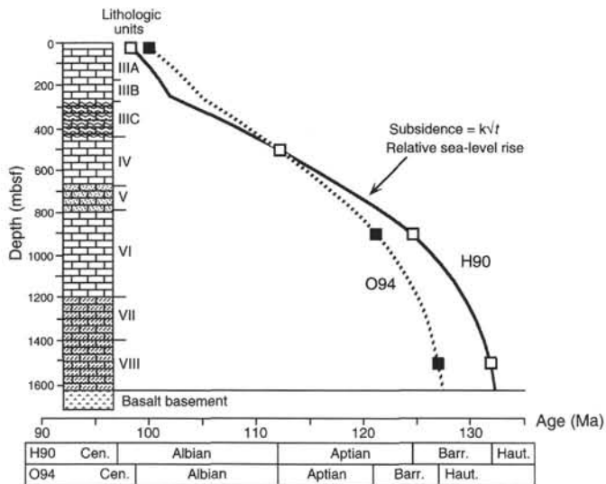
Figure 14. Inferred Early Cretaceous subsidence curves for Hole 866A. Two curves are shown that correspond to the time scales of Harland et al. (1990, "H90") and Obradovich (1994, "O94"). Age control points are from the Sr-isotopic data of Jenkyns et al. (this volume). The equation, \text{depth} = k\sqrt{t} is shown for each curve. Roman numerals at the left denote lithologic units used in the site report (Shipboard Scientific Party, 1993c).
