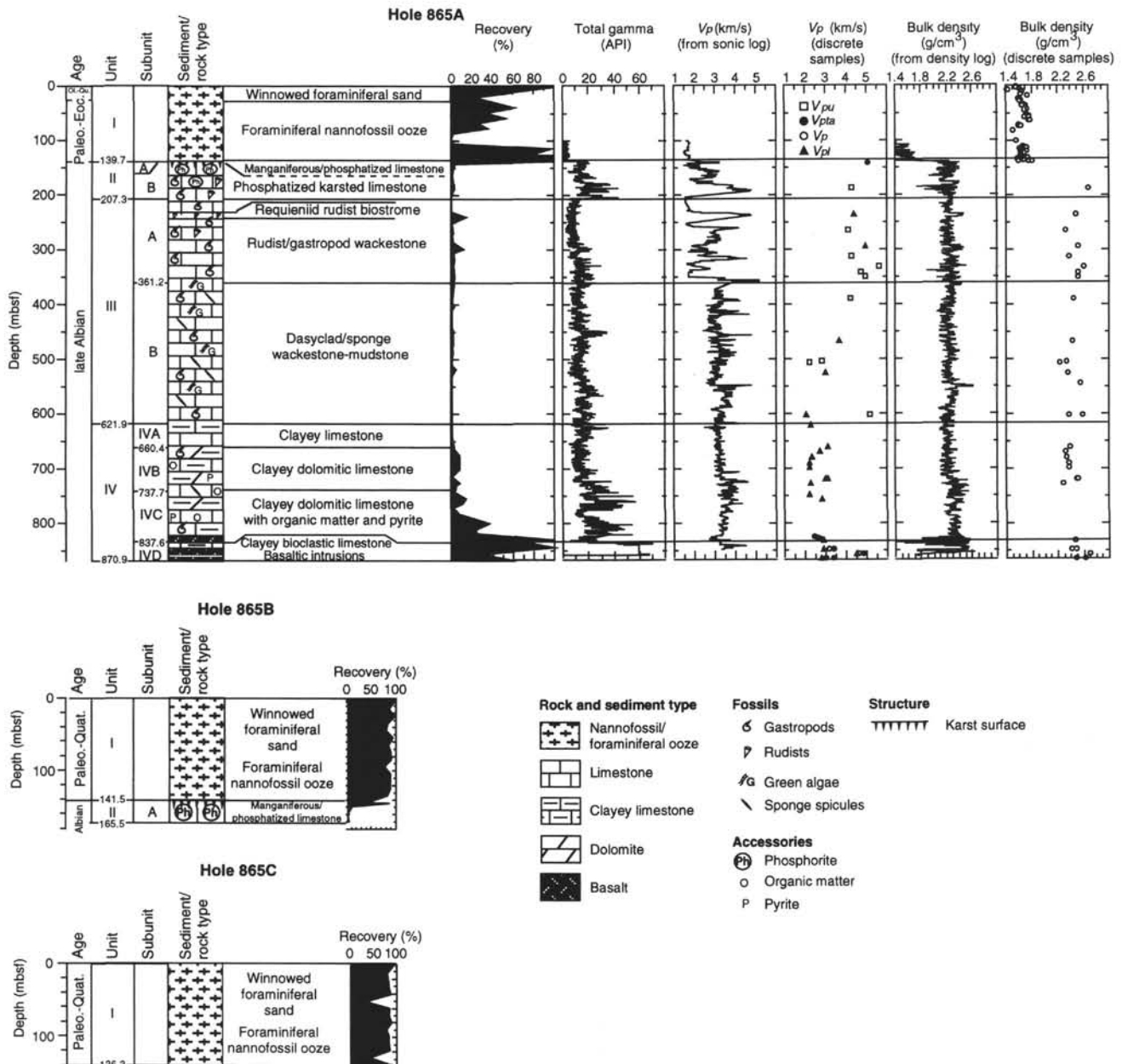
Figure 4. Summary of lithologic units, biostratigraphic dates, physical properties, and logging data from Site 865. Measurements of discrete sample P -wave velocities are labeled by orientation: V_{pu} is unoriented; V_{pta} and V_{ptb} are transverse (horizontal); and V_{plv} is longitudinal (parallel to core axis) (from Shipboard Scientific Party, 1993a).
