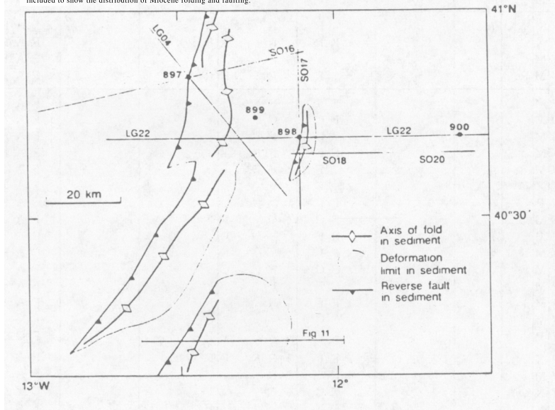
Figure 2. Location map of the line drawings of interpreted seismic lines shown on Figure 3. Part of the structural map of Masson et al. (1994) is included to show the distribution of Miocene folding and faulting.
