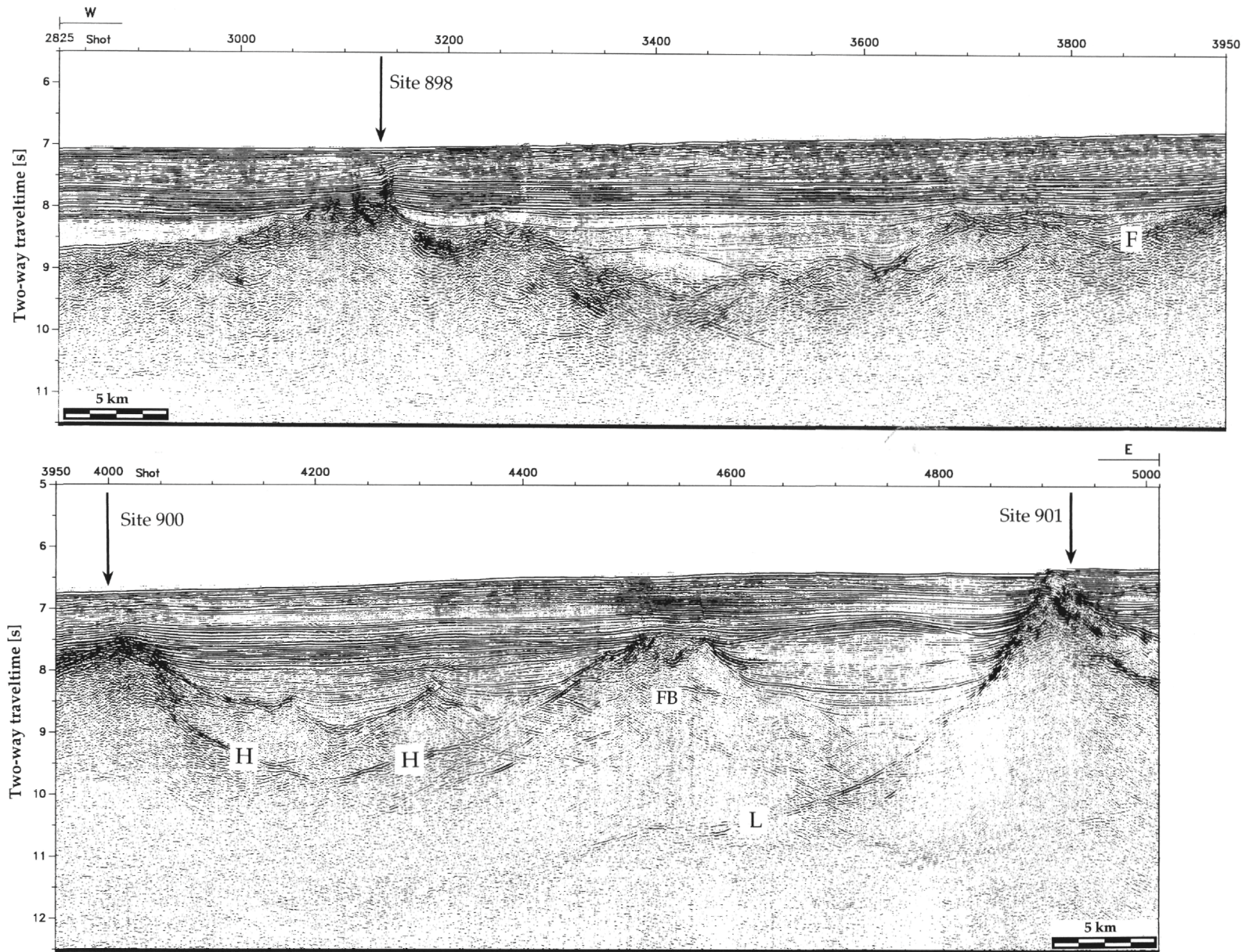
Figure 3. Time-migrated seismic section of profile LG12 covering (from west to east) Sites 898-901 (50-m shot spacing; vertical exaggeration 2). Interpretations based on the depth section in Figure 8 are presented in Figure 10. Note the detachment fault H, the listric fault structure L, and the low-angle fault F. FB = fault block.
