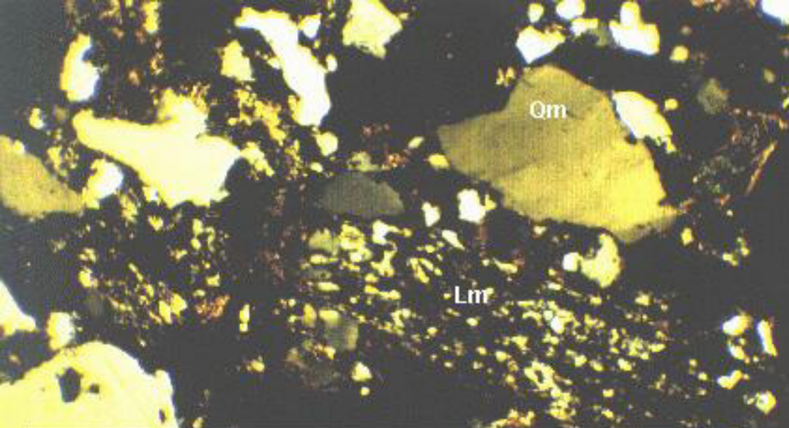
Metamorphic lithic (Lm) and angular monocrystalline quartz (Qm) in medium-grained carbonate-cemented sandstone. Cross-polarized light. Sample 159-959D-76R-2, 0-3 cm
