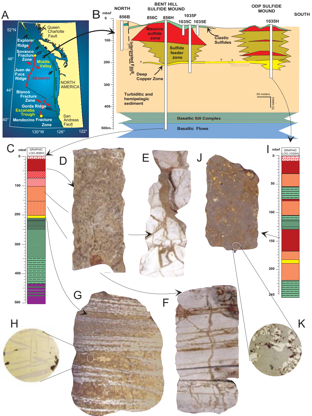
A. Location map showing the tectonic setting of the sediment-covered spreading centers at Middle Valley and Escanaba Trough on the Juan de Fuca-Gorda spreading system (modified from Davis, Mottl, Fisher, et al., 1992). B. North-south cross section of the BHMS deposit and ODP Mound (red), the underlying sulfide feeder zones (olive green), the Deep Copper Zone (yellow), host turbiditic and hemipelagic sedimentary rocks, and underlying basaltic sills and flows. C. Stratigraphic section for Hole 856H showing the distribution of mineralized and nonmineralized subunits. Red shades = massive sulfide, hatched yellow = feeder zones, thin yellow band at 200 mbsf = the Deep Copper Zone, green = sediment, and purple = basalt. D. Massive, vuggy pyrite-pyrrhotite. E. Subvertical single and multiple (ribbed) massive sulfide veins composed of pyrrhotite, isocubanite, chalcopyrite, pyrite, magnetite, and anhydrite cutting hydrothermally altered sedimentary rock. F. Pyrrhotite and sphalerite as bedding-parallel veins and replacements, subvertical veins, and disseminations and blebs in graded turbiditic sandstone. G. Sulfide-banded cross-laminated sandstone. Horizontal veinlets and impregnations of Cu-rich sulfides and Mg-rich chlorite have filled pore space and replaced sandstone. H. Photomicrograph of crystallographically oriented lamellar intergrowth of chalcopyrite (gray) within isocubanite (yellow). I. Stratigraphic section for Hole 1035H. Red = massive sulfide, hatched yellow = feeder zones, and green = sediment. J. Sphalerite-rich ore with pyrite and chalcopyrite. K. Photomicrograph of sphalerite (dark gray) and pyrite (light gray).
