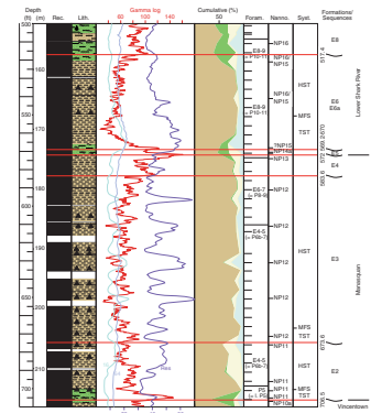
F5. Summary stratigraphic section, lower Shark River and Manasquan Formations, p. 44.
