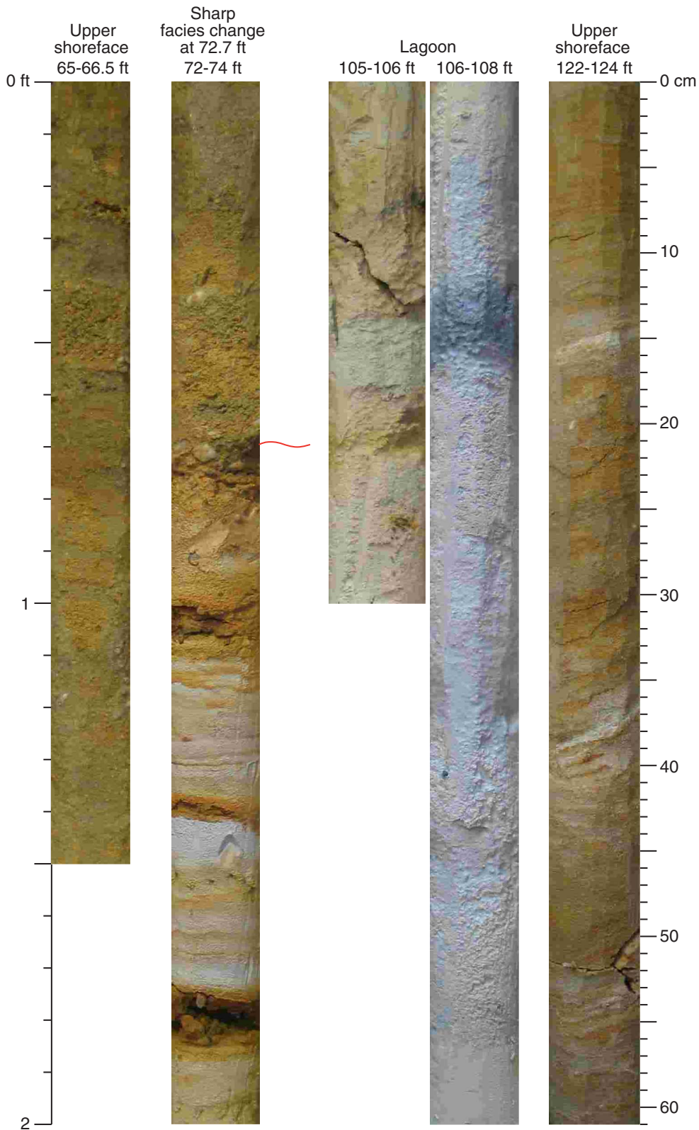
Figure AF1. Representative lithofacies from the Double Trouble corehole: upper shoreface sediments from the Cohanse Formation (65–66.5 ft; 19.8–20.3 m); sharp surface at 72.7 ft (22.2 m) in the Cohanse Formation; lagoonal facies in the Cohanse Formation (105–106 ft and 106–108 ft; 32.0–32.3 and 32.3–32.9 m); and upper shoreface facies in the Kirkwood Formation (122–124 ft; 37.2–37.8 m).
