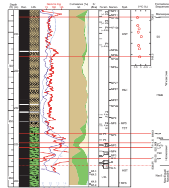
F6. Summary stratigraphic section Vincentown, Hornerstown, and New Egypt/Navesink Formations, p. 45.
