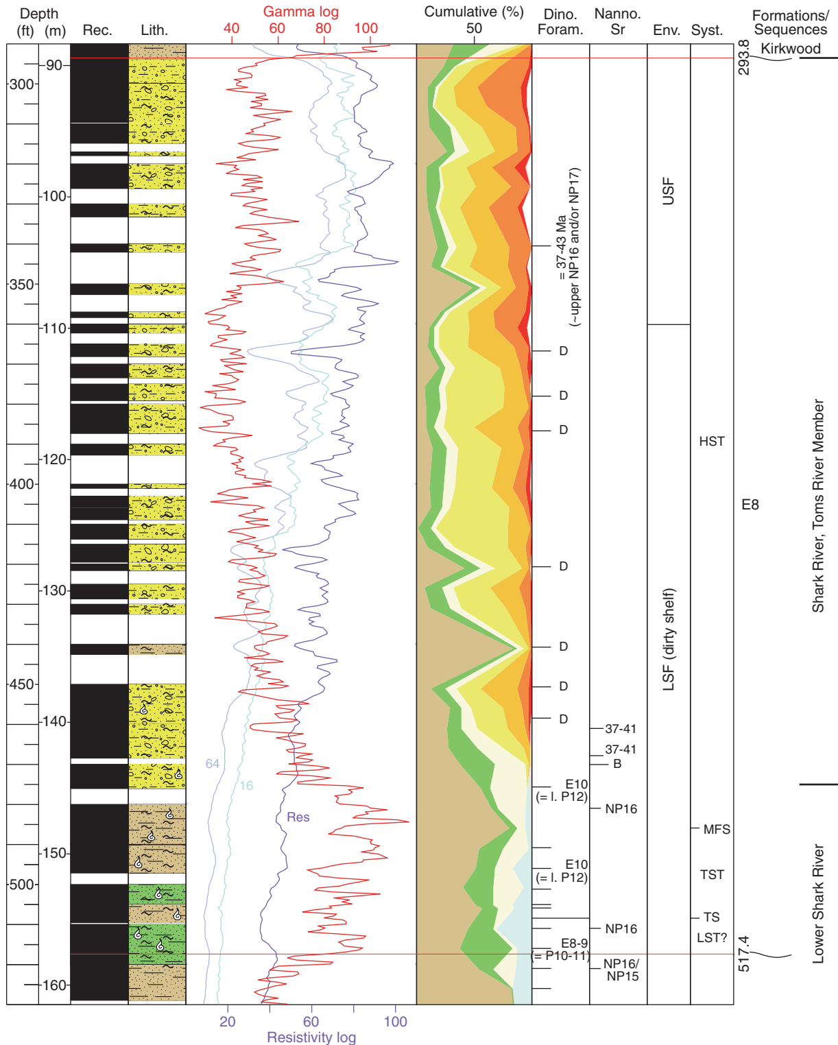
Figure F4. Summary stratigraphic section for the Toms River Member of the Shark River Formation (upper middle Eocene) from the Double Trouble borehole. with core recovery (Rec.), lithology (Lith.), gamma ray and resistivity log signatures, age, and environments (Env.). Dino. = Dinocyst zone, Foram. = foraminifer zone, Nanno. = nannofossil zone, Sr = strontium age estimate (Ma), Syst. = systems tract. Lines Res, 16, and 64 are all resistivity logs. NP Zones are from Martini (1971) and Martini and Müller (1986). E and P Zones are from Berggren et al. (1995). E8 is a sequence defined by Browning et al. (1997a, 1997b). See Figure F2B for legend.
