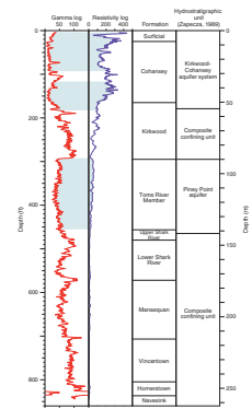
F7. Lithologic and hydrostratigraphic terminology, p. 46.
