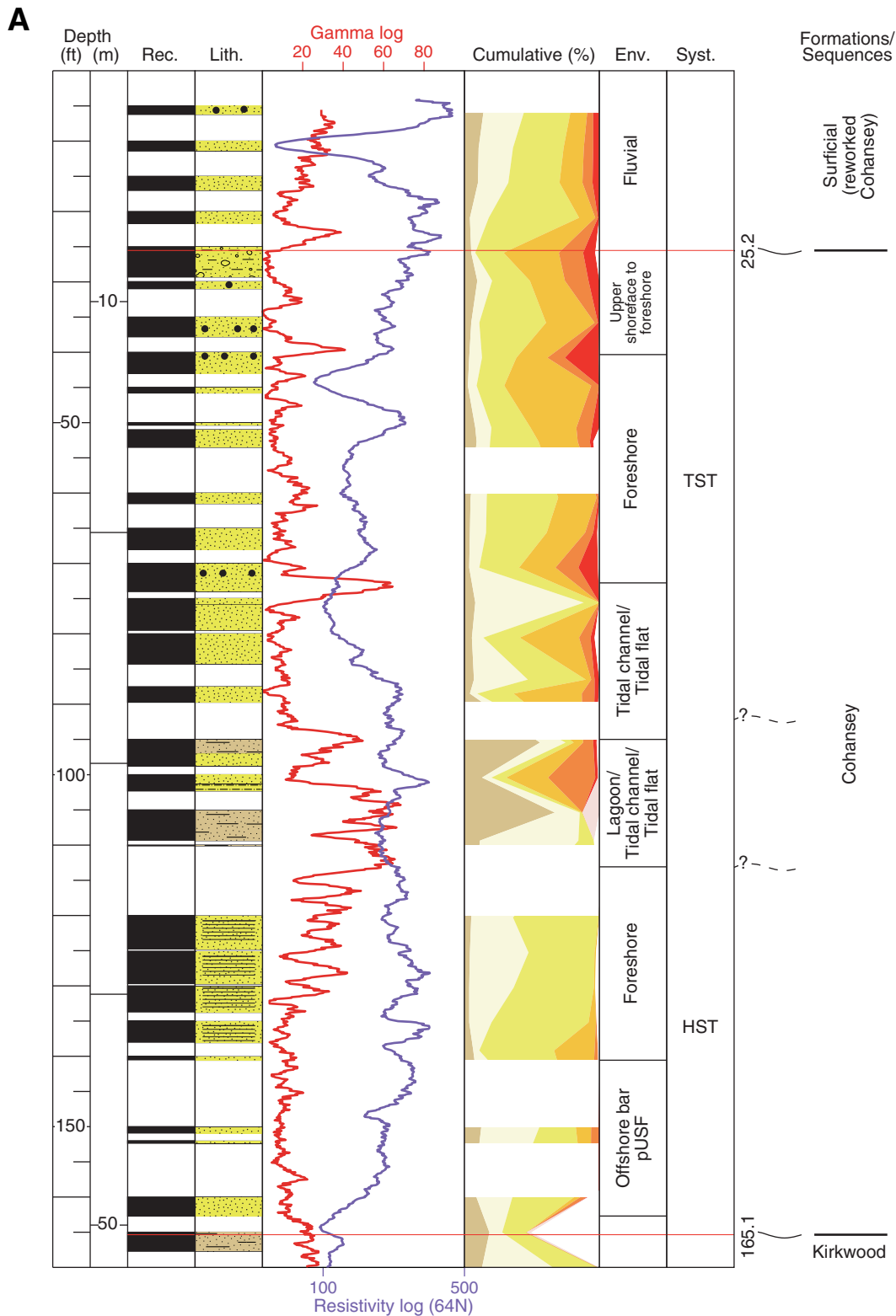
Figure F2. A. Summary stratigraphic section for the Cohanse Formation (?uppermost middle to late Miocene) in the Double Trouble borehole, with core recovery (Rec.), lithology (Lith.), gamma ray and resistivity log signatures, age, and environments (Env.). Syst. = systems tract. See part B for legend. (Continued on next page.)
