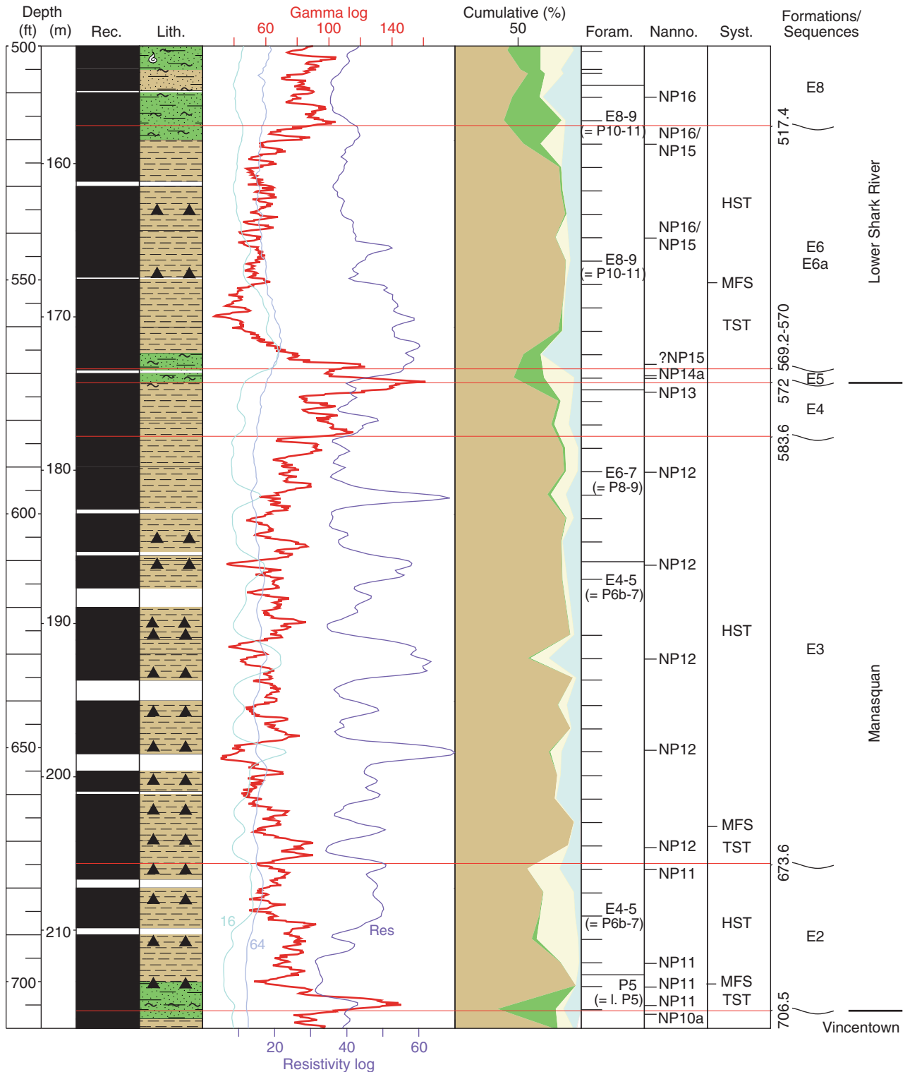
Figure F5. Summary stratigraphic section for the lower Shark River (middle Eocene) and Manasquan (lower Eocene) formations from the Double Trouble borehole, with core recovery (Rec.), lithology (Lith.), gamma ray and resistivity log signatures, and age. Foram. = foraminifer zone, Nanno. = nannofossil zone, Syst. = systems tract. Lines Res, 16, and 64 are all resistivity logs. E and P Zones are from Berggren et al. (1995). NP Zones are from Martini (1971) and Martini and Müller (1986). E2–E5 and E8 are sequences defined by Browning et al. (1997a, 1997b). See Figure F2B for legend.
