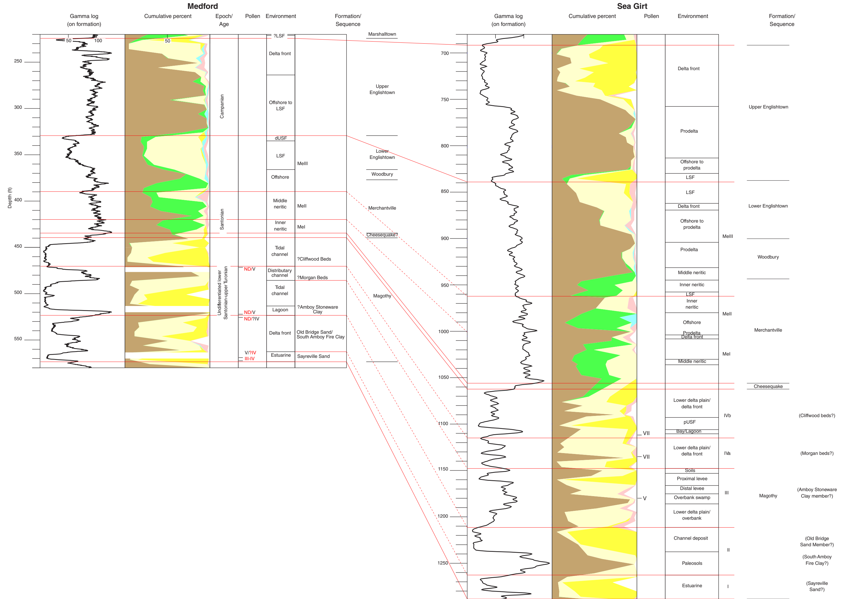
Medford Site Chapter, Figure 11. Strike section showing the relationships between the Turonian to lower Campanian sequences discussed in text. Red lines = sequence boundaries. LSF = lower shoreface, dUSF = distal upper shoreface, pUSF = proximal upper shoreface.
