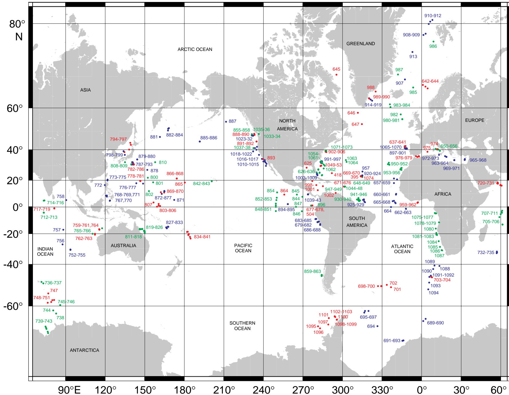
ODP Legs 100-178, Sites 625-1103
