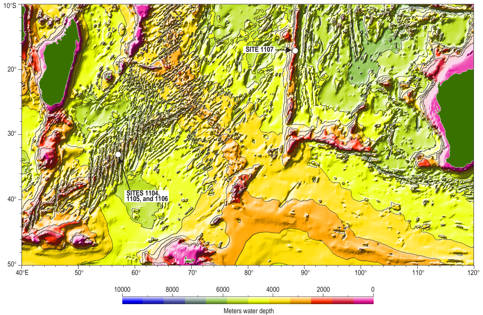
Bathymetry model of the Indian Ocean showing Sites 1104, 1105, and 1106 on the east wall of the Atlantis II Fracture Zone of the Southwest Indian Ridge and Site 1107 on the Ninetyeast Ridge. Modified from an image acquired from the Delft University of Technology altimetry interactive World Wide Web page ( http://www.deos.tudelft.nl/altim/ceo/pim.html ).
