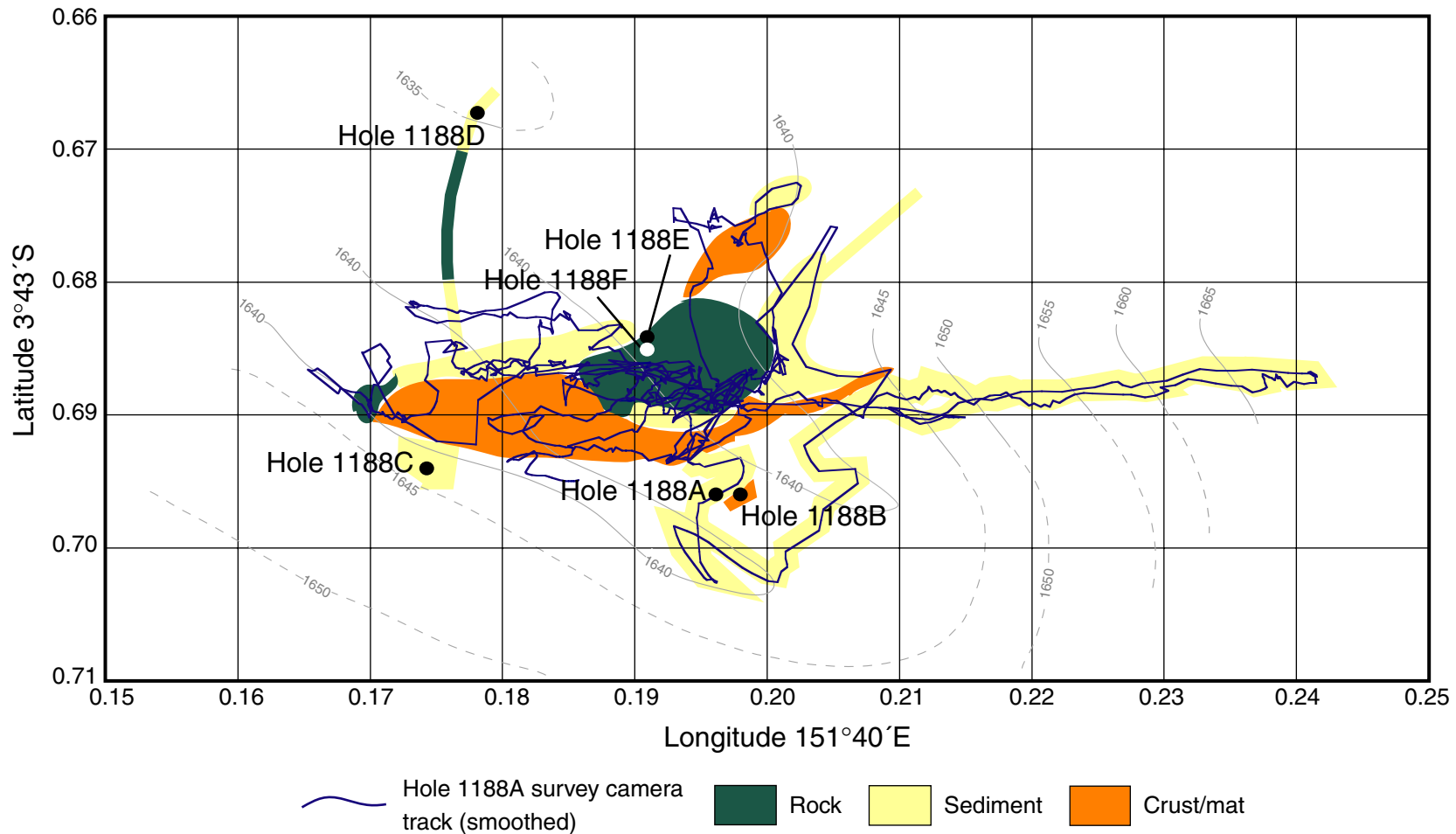
Figure F8. Calculated course of vibration-isolated television (VIT) survey during the site survey prior to spudding of Hole 1188A and observed seafloor character. Bathymetric contours (5-m intervals) within the survey area are based on VIT cable measurement and sonar altimetry, calibrated to the actual drill pipe measurement depth of Hole 1188A. Contours outside the survey area are derived from submersible dives and have been added to show the general shape of Snowcap. Only the track from the initial survey is shown, but additional seafloor cover information from other surveys has been added. Global Positioning System averaged locations for all of the ODP holes at Site 1188 are also shown.
