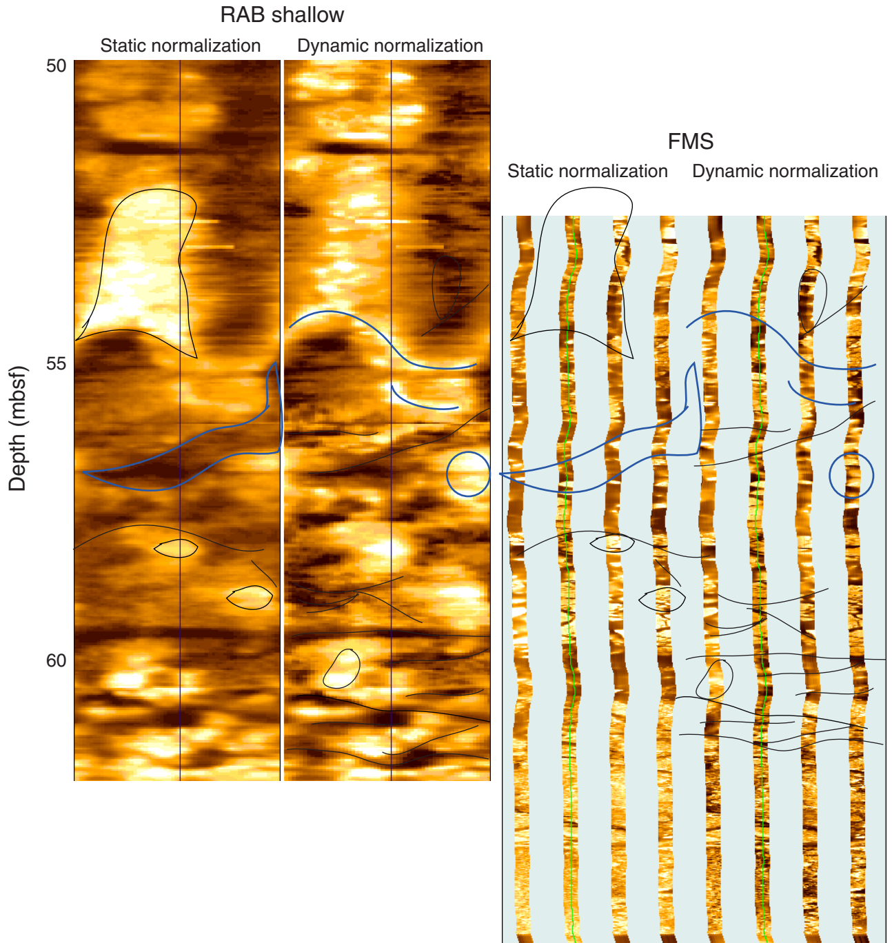
Figure F37. Comparison between resistivity at the bit (RAB) and Formation MicroScanner (FMS) images in Hole 1189C.
