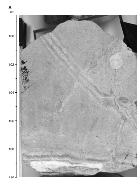
F24. Photograph and sketch of complex vein relationships, p. 58.
