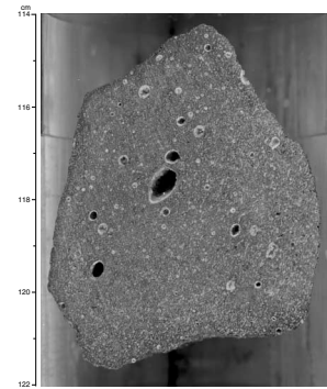
F28. Moderately vesicular aphyric volcanic rock, p. 65.
