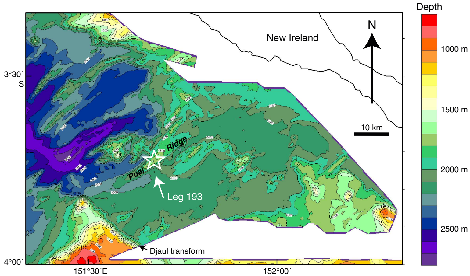
Figure F4. Bathymetry of the Eastern Manus Basin from multibeam data compiled by Institut Francais de Recherche pour l'Exploration de la Mer (IFREMER). The southeast-trending Djaul transform is conspicuous. The northeast-trending deep on the western side is a failed spreading segment. The PACMANUS hydrothermal field lies at the crest of a northeast-trending ridge of dacite (Pual Ridge).
