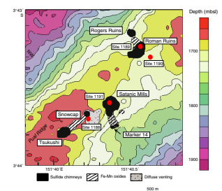
F7. Distribution of hydrothermal deposits within the PACMANUS field, p. 38.
