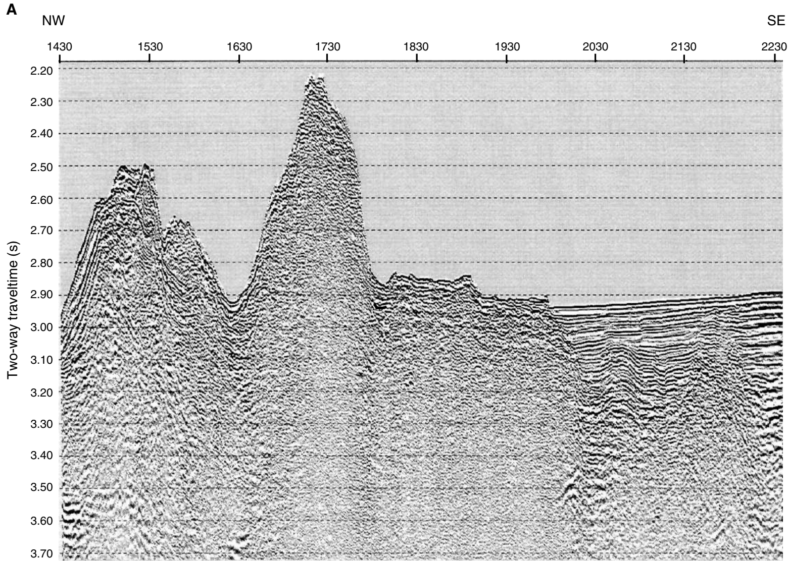
Figure F5. A. High-resolution single-channel seismic profile of the section across Pual Ridge at the position of the PACMANUS hydrothermal field. All Leg 193 sites lie on the crest of Pual Ridge. Data from the Somme cruise 94, Leg 2, single channel seismic line 07. (Continued on next page.)
