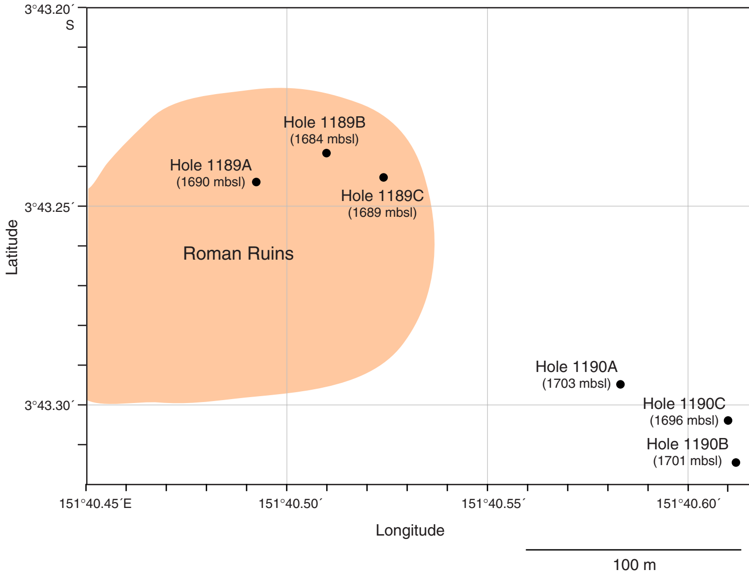
Figure F25. Hole locations for Sites 1189 and 1190. Shaded area around Site 1189 (Roman Ruins) = the approximate area of outcrop of chimney structures mapped by submersible and camera tow.
