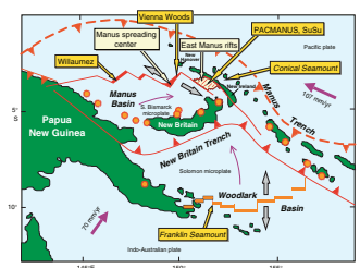
F2. Regional tectonic setting of the PACMANUS hydrothermal field drilled, p. 32.
