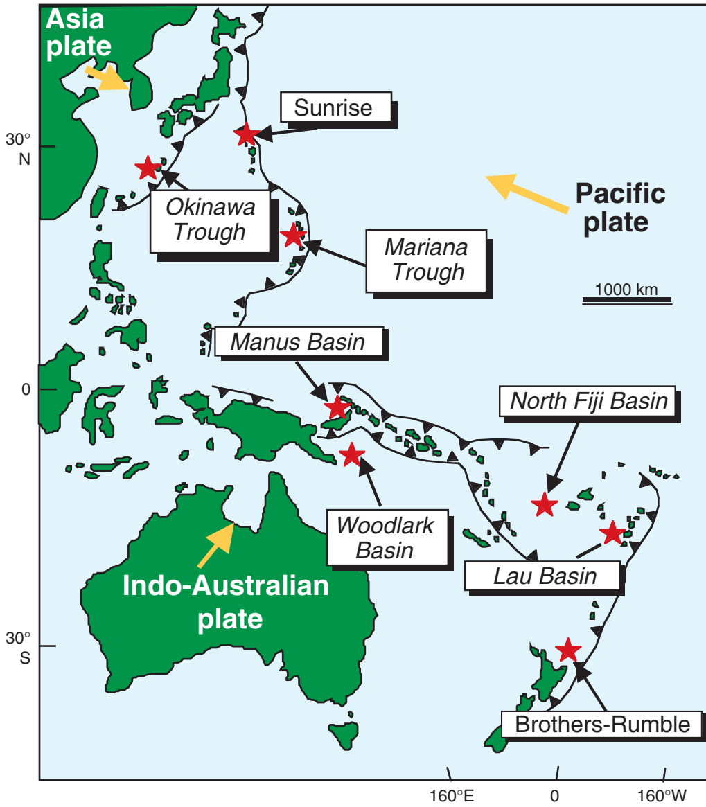
Figure F1. Major active hydrothermal sites at convergent margins of the western Pacific Ocean. Large arrows = plate movements.
