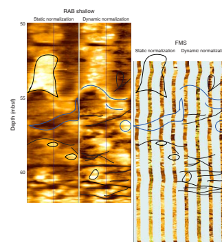
F37. Comparison between RAB and FMS images in Hole 1189C, p. 76.
