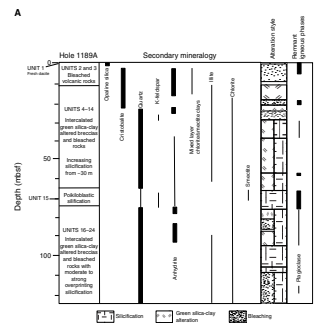
F29. Summary of lithostratigraphic units, alteration style, and distribution of major and minor to trace alteration phases for Holes 1189A and 1189B, p. 66.
