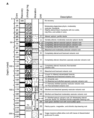
F10. Graphic summary log for Holes 1188A and 1188F showing the lithologic characteristics of the various units including alteration, p. 41.
