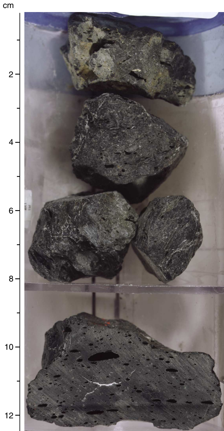
Figure F11. Close-up photograph of fresh, black, moderately vesicular rhyodacite from the upper part of Hole 1188A (interval 193-1188A-4R-1, 0-12.5 cm).
