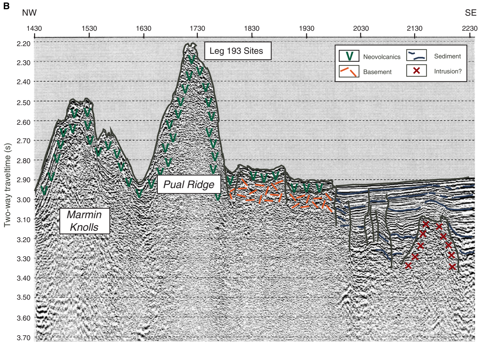
Figure F5 (continued). B. The interpretation of the high-resolution single channel seismic profile of the section across Pual Ridge.
