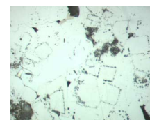
F34. Sphalerite or magnetite precipitated on early pyrite and overgrown by later pyrite, p. 73.
