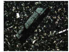
F12. Fresh plagioclase phenocryst set in groundmass, p. 44.
