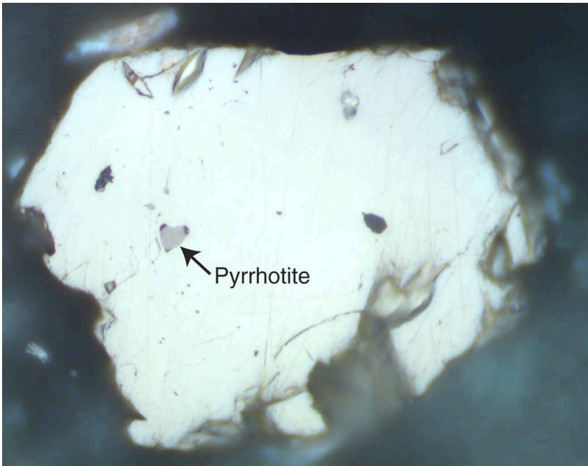
Figure F22. Photomicrograph in reflected light of pyrrhotite inclusion (diameter = 0.006 mm) with smaller magnetite inclusions in pyrite (Section 193-1188F-1Z-3 [Piece 3, 86–89 cm]; width of view = 0.14 mm. Photomicrograph ID# 1188F_06, thin section 61 ).
