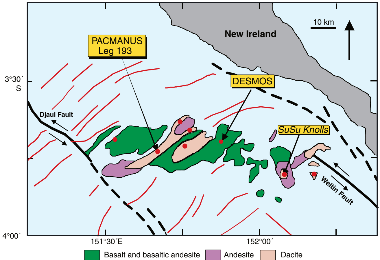
Figure F6. Seafloor geology of the Eastern Manus Basin. Edifices of the eastern Manus volcanic zone, which extends between the active ends of the Djaul and Weitin transform faults, range from picritic basalt to rhyodacite in composition. Red dots = known hydrothermal sites, including the three main active sites of PAC-MANUS, Deep Sea Monitoring System (DESMOS), and SuSu Knolls. Red lines = extensional fault scarps.
