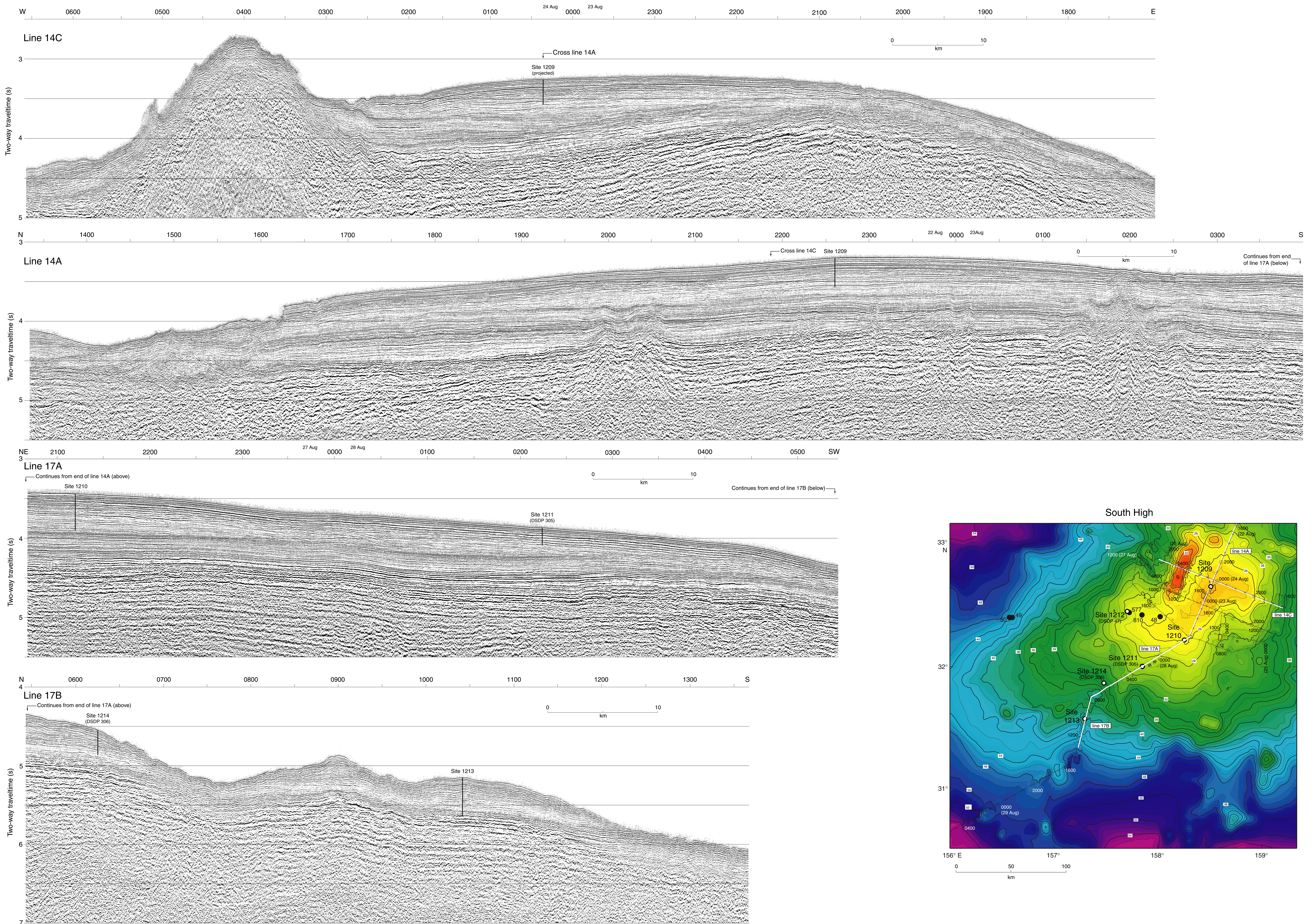
Chapter 11, Figure F8. Seismic lines (14A, 14C, 17A, and 17B) collected over the South High showing the locations of Sites 1209, 1210, 1211, 1213, and 1214 (Site 1212 is not located on one of our seismic lines). Bathymetric map shows the locations of all the South High seismic lines collected. Seismic lines not displayed in this figure (14B, 14D, 15, 16, 17C, and 17D) are shown in Figures F13, p.19, and F14, p.20.
