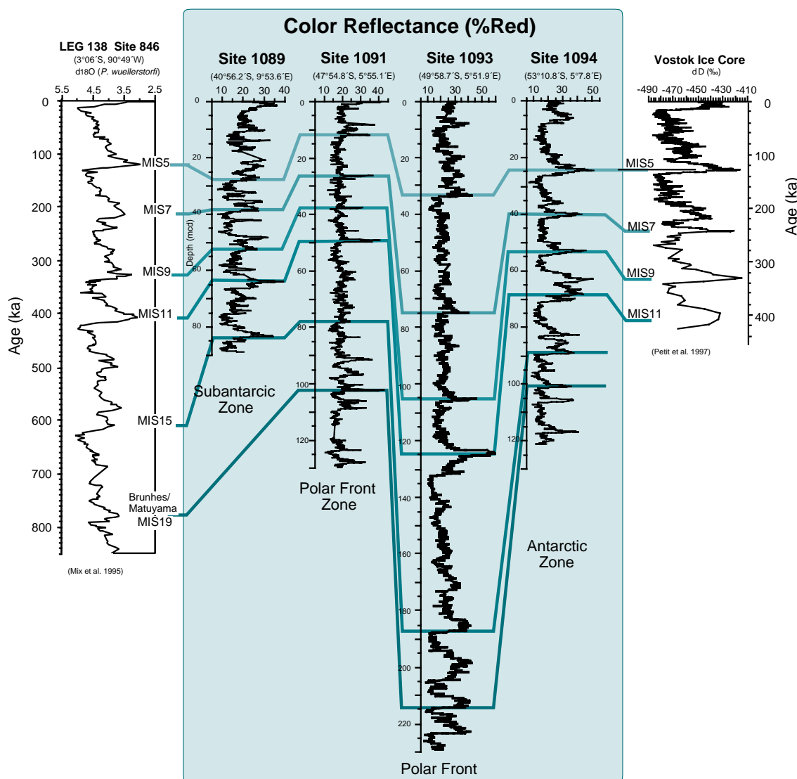
Figure 3: Correlation of percent red reflectance (650-750 nm) among Leg 177 Sites 1089, 1091, 1093 and 1094 along a north-south transect across the ACC. Peaks in color reflectance, reflecting increased carbonate content, have been correlated to the transitions between marine isotope stages of the late Pleistocene as expressed in the oxygen isotope record of Site 846 (Mix et al., 1995). Also shown is the deuterium isotopic record of the Vostok Ice Core for the last four climatic cycles (Petit et al., 1997).
