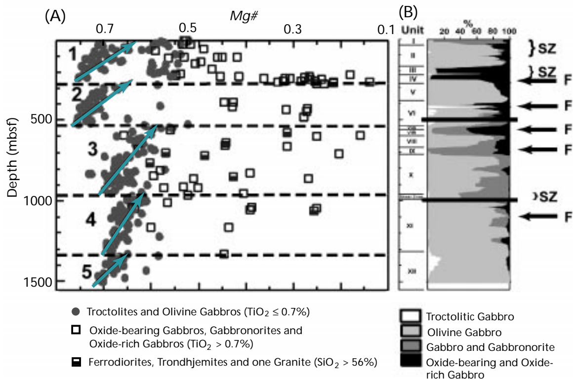
Figure 2: Chemical- and lithostratigraphic summary of Hole 735B. Data are from Robinson et al. (1989), Dick et al. (in press), and J. Hertogen (unpublished). A. Mg# versus depth ( Mg\# = Mg / ([Mg + Fe^{2+}]) , assuming that Fe^{2+} / [Fe^{2+} + Fe^{3+}] = 0.86 ). Dashed lines at bases of major breaks in compositional trends define five principal plutonic masses within the drilled section, each becoming more differentiated (proportionally iron-rich) upward, as indicated by the diagonal arrows. All other samples represent narrow, cross-cutting facies each typically 5-15 cm thick. B. Simplified summary of the lithostratigraphy giving the main lithologic units defined during Legs 118 and 176, proportions (%) of intervals of principal lithofacies constructed using a rolling average at 20-m intervals, and structure. (SZ = shear zone, F = fault.) Horizontal lines are drawn across the lithofacies summary at 500-m intervals.
