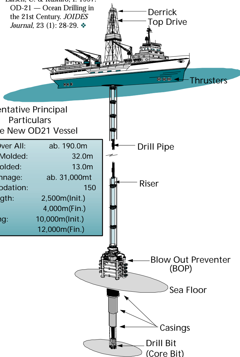
Figure 3: Artist's Drawing of the OD-21 Riser Drillship.
