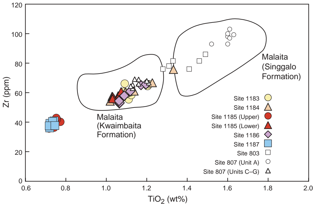
Figure 3. Zr vs. TiO 2 data for basement rocks recovered at the Leg 192 sites, and ODP Sites 803 and 807. Fields for basaltic lava flows of the >2.7-km-thick Kwaimbaita Formation and the overlying ~750-m-thick Singgalo Formation on Malaita are shown for comparison. [Editor's Note: Figs. 2 and 4 are in the article. on pages 3 and 4.]
