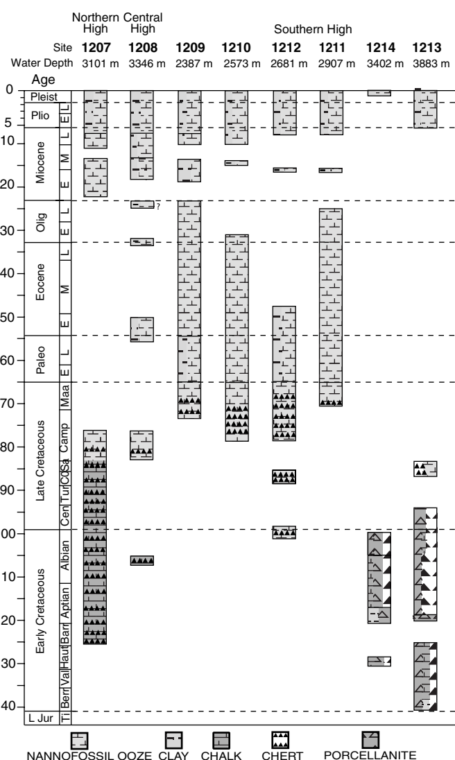
Figure 2. Summary of stratigraphy and lithologic succession from Sites 1207 to 1214. Lithology is plotted against time to show duration of periods of deposition and location of unconformities. Southern High Sites 1209 to 1214 are arranged by water depth.
