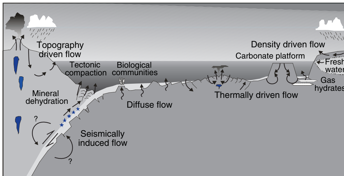
Figure 1. Schematic diagram showing the involvement of subseafloor fluid flow systems in a variety of geologic processes (modified from a figure courtesy of Earl Davis).
