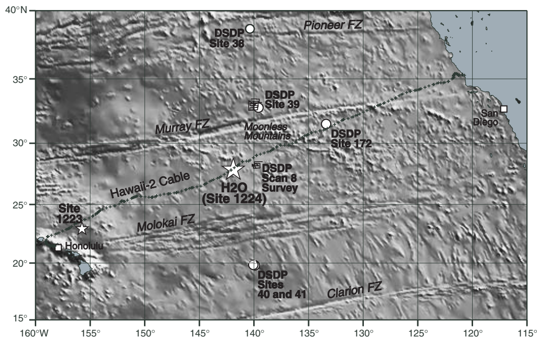
Figure 1. The repeater locations of the Hawaii-2 cable (plus signs), the Nuuanu landslide drill site (Site 1223, small star), the location of the H2O junction box and drill site (Site 1224, large star), and the location of previous drilling on Legs 5 and 18 of DSDP are shown. Superimposed on the map is the satellite derived bathymetry. The locations of the major fracture zones are marked.
