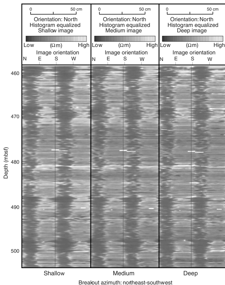
Figure 4. Borehole breakouts observed using RAB (Resistivity at the Bit) images in Hole 808I at 460 to 505 mbsf. Resistivity values decrease with increasing darkness. Vertically aligned dark belts represent borehole breakouts that indicate orientation of the minimum horizontal compressive stress is ~northeast-southwest. This orientation is in good agreement with the plate convergence vector.
