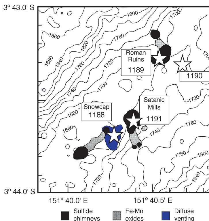
Figure 2. Distribution of hydrothermal deposits along the crest of Pual Ridge, and location of Leg 183 sites (stars). Bathymetry in meters.
