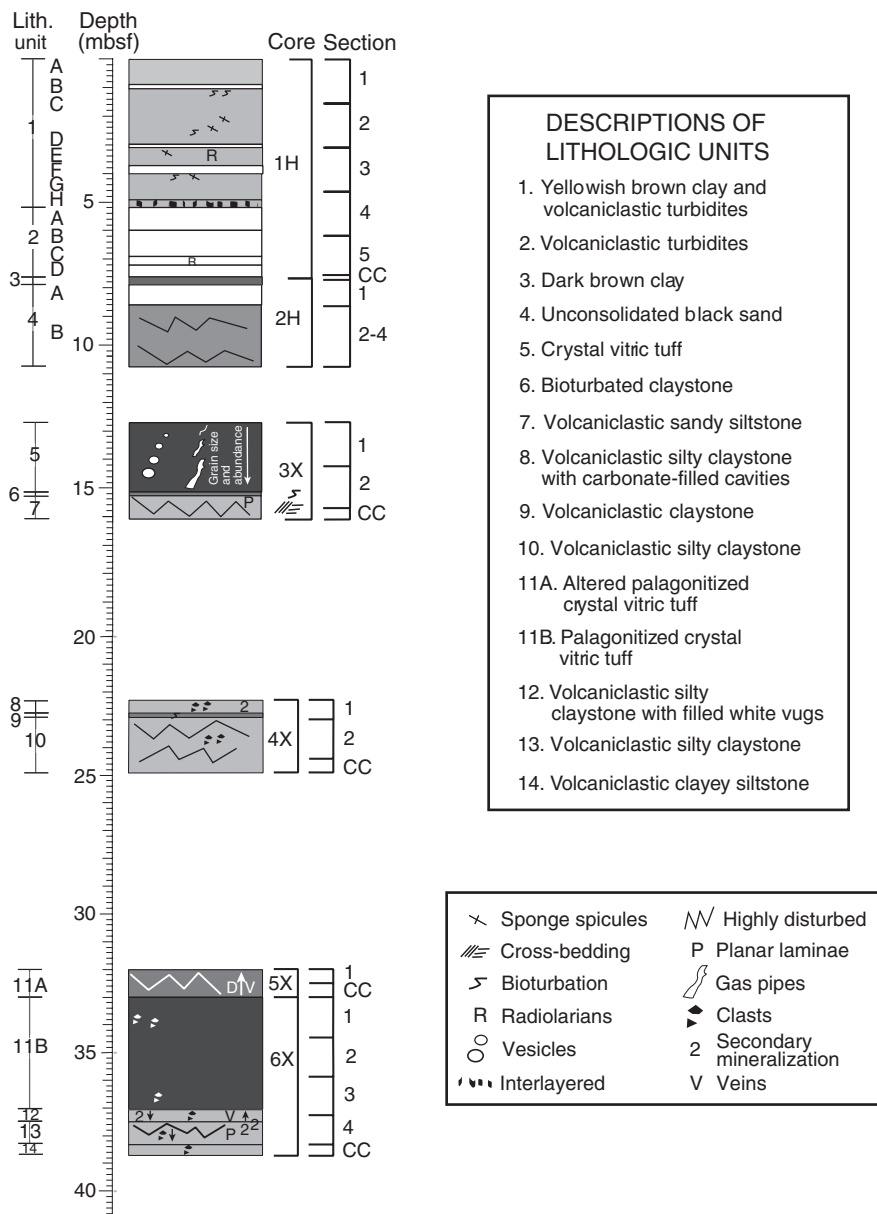
Figure 3. Lithological units of Hole 1223A. The crystal vitric tuffs (Units 5 and 11) appear to have been deposited at the seafloor at temperatures exceeding 200°C. This suggests that the Nuuanu Landslides were accompanied by pyroclastic activity similar to the Mount St. Helens eruption in 1990 but an order of magnitude larger.
