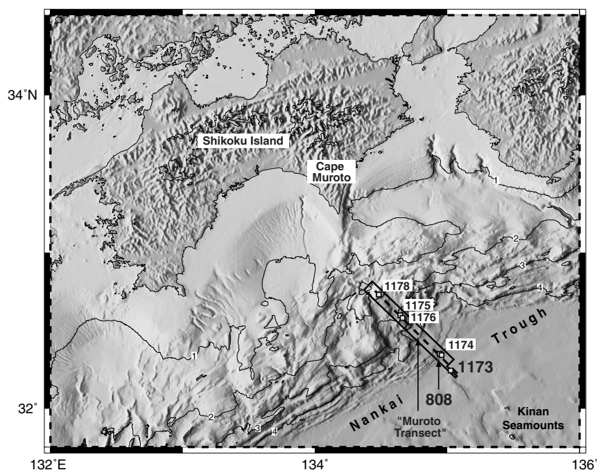
Figure 1. Map showing sites drilled along the “Muroto Transect” during ODP Leg 131 (Site 808) and Leg 190 (Sites 1173-1176, 1178), and revisited during Leg 196 (Sites 808 and 1173). The box surrounding the numbered drilling sites outlines the three-dimensional seismic survey conducted by the R/V Maurice Ewing in 1999.
