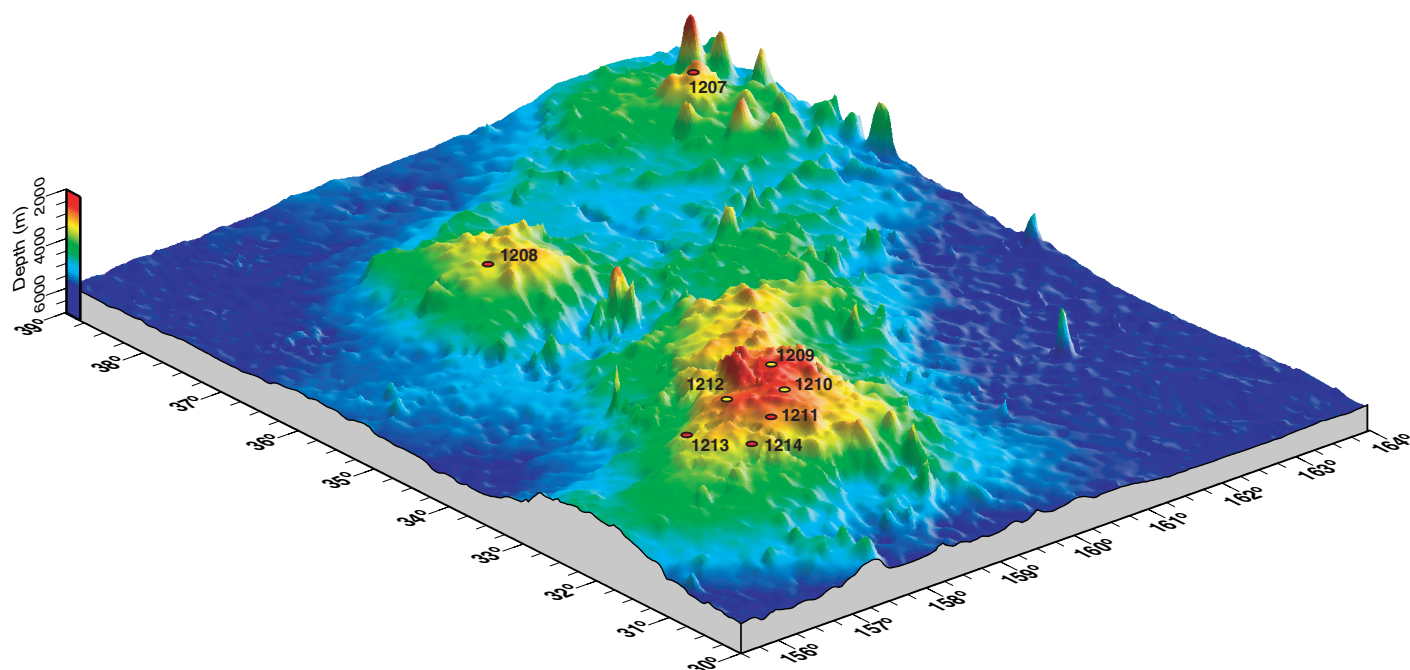
Figure 1. Bathymetric map of Shatsky Rise in the Northwest Pacific Ocean showing locations of Leg 198 drill sites. Site 1207 is located on the Northern High, Site 1208 is on the Central High, and Sites 1209 to 1214 are on the Southern High. Altimetry-derived bathymetry from Smith and Sandwell (1997).
