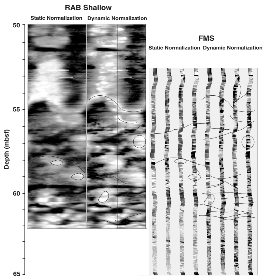
Figure 3. Comparison of resistivity images of the borehole wall obtained by logging-while-drilling (LWD) resistivity-at-bit (RAB), and by formation microscanner (FMS) during subsequent wireline logging of Hole 1189C. Correlated features are marked.
