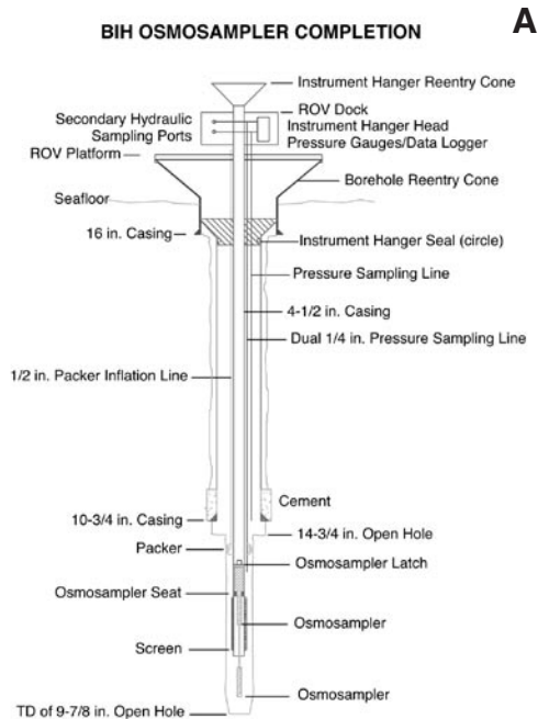
Figure 5. A. Schematic diagram of a Borehole Instrument Hanger (BIH) osmosampler installation, also known as a CORK-II, used to monitor subsurface fluid circulation, pressure, and temperature (Graber et al., 2002; Jannasch et al., in press). The BIH is installed in a borehole reentry cone that has 16 in and 10-3/4 in casing set in the hole. A single packer is used to seal off zones of open hole below the casing; a formation fluid sampling screen is mounted on the outside of the casing. The removable osmosampler package is latched in below the packer so that one of the samplers extends into open hole. Head design and sampling and data port locations are similar to the ACORK. B. Head assembly of the CORK-II above the landing platform installed in Hole 1255A in the Costa Rica Trench during ODP Leg 205 in 2002 (Jannasch et al., in press). The observatory was visited by DSV Alvin later in 2002 for sampling; note the underwater mateable connector visible at the forward end of Alvin's basket in the foreground of the image (Video still courtesy of WHOI).
