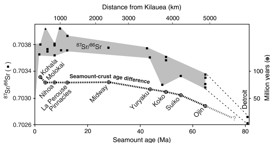
Figure 2. Compositional changes in magmas produced by the Hawaiian hotspot through time. The shaded field shows the range of published ^{87}\text{Sr}/^{86}\text{Sr} of tholeiitic basalts vs. age and distance along the Hawaiian-Emperor chain. Note that data from Detroit Seamount are significantly less radiogenic than at younger volcanoes. The circles connected by the thick dotted line show the trend in age difference between seamounts and the underlying ocean crust (from Keller et al., 2000).
