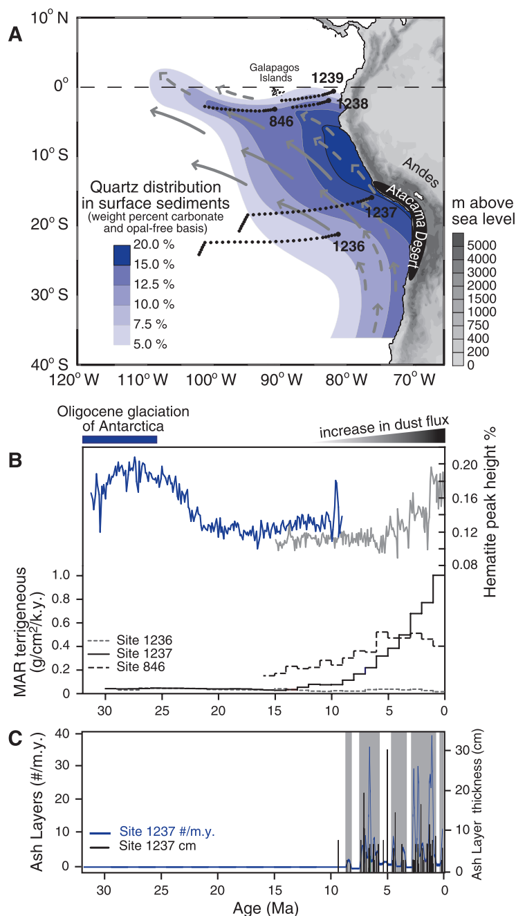
Figure 2. A. Quartz distribution in surface sediments of the subtropical southeast Pacific, expressed as weight percentage (carbonate- and opal-free basis; Molina-Cruz, 1977). Gray arrows indicate trade winds. Sites 1236, 1237, 1238, and 1239 (Leg 202), and Site 846 (Leg 138) are shown with their plate tectonic backtracks at 1 m.y. intervals. B. Siliciclastic accumulation rates and hematite peak height at Sites 1236 (gray line) and 1237 (blue line). Accumulation rates of siliciclastics were estimated at 1 m.y. intervals as the product of (100% - wt% CaCO 3 - wt% organic matter - wt% biogenic opal), sedimentation rate, and dry bulk density. The hematite peak height is derived from color reflectance spectra (550 nm peak above background) and serves as a rough proxy for changing concentrations of hematite. C. Ash frequency at Site 1237 (#/m.y., blue line), calculated as the first derivative of the cumulative number of ash layers vs. age. Vertical bars indicate the age and thickness (cm) of individual ash layers.
