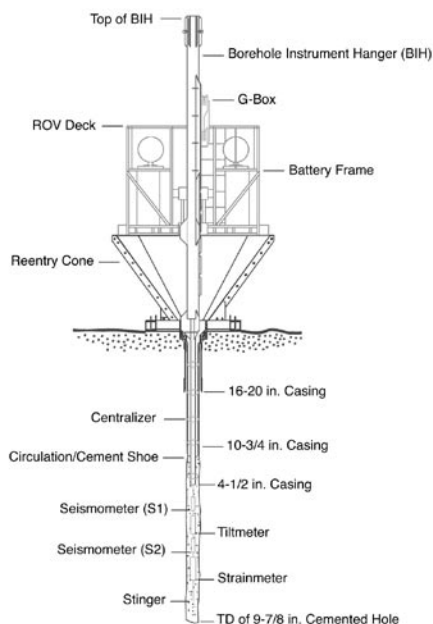
BIH STRAIN-TILT-SEISMOMETER COMPLETION
