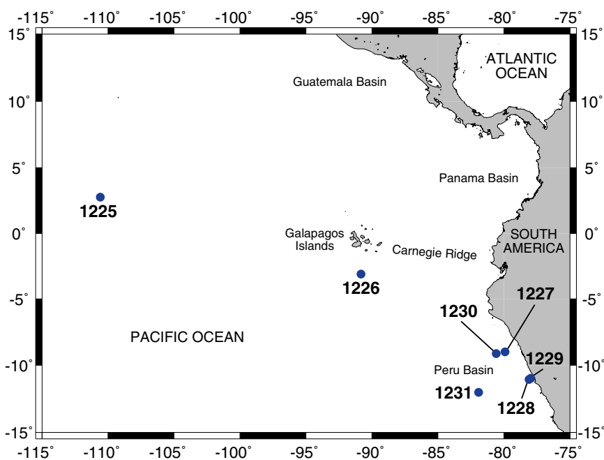
Figure 1. Location map of seven ODP Leg 201 drillsites off Peru.
