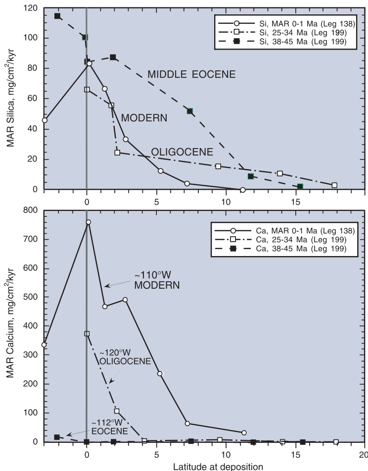
Figure 3. Calcium and silica mass accumulation rates (MAR) profiles for the Pleistocene (0 to 1 Ma), Oligocene, and middle Eocene. Late Pleistocene data are from Farrell et al. (1995).
