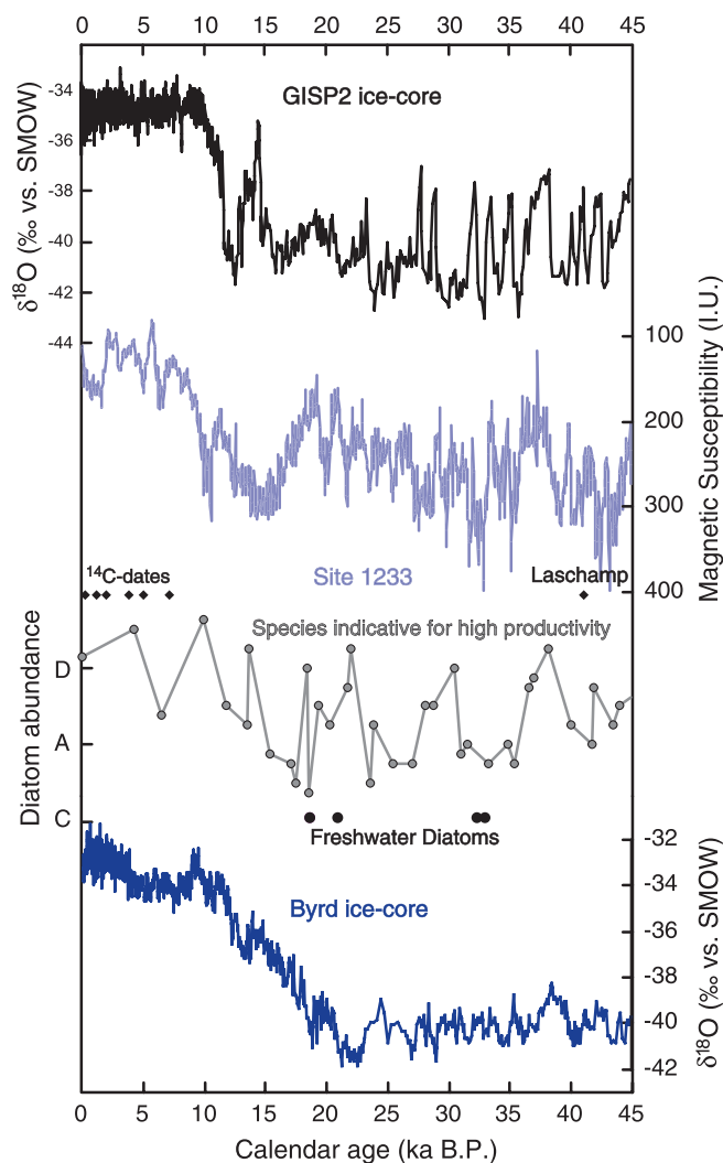
Figure 4. Millennial-scale variability at Site 1233. Magnetic susceptibility and diatom abundance plotted on a preliminary age scale for the interval 0 to 45 ka. The age scale is based on Holocene age control points derived from a correlation of the magnetic susceptibility records between Site 1233 and AMS- ^{14}\text{C} dated core GeoB 3313-1 (Lamy et al., 2002) and the location of the Laschamp Event. All ages are calendar years before present (B.P.) and are linearly interpolated between the dates, resulting in substantial uncertainty between 9 and 40 ka. General character of variability at Site 1233 is similar to isotopic variability in the GISP2 ice core in Greenland and the Byrd ice core in Antarctica. Both ice core records are plotted on the GISP2 time scale (Blunier and Brook, 2001). SMOW=oxygen isotopic composition of standard mean ocean water.
