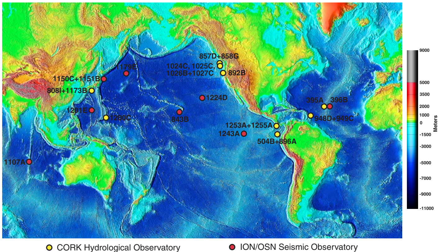
Figure 1. ODP borehole observatories installed in ODP/DSDP reentry holes. Mercator projection of digital bathymetry and topography data from National Geophysical Data Center (2000).
