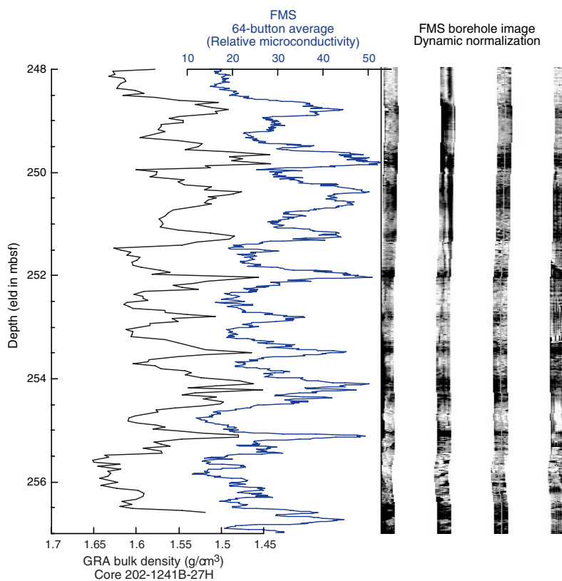
Figure 3. Pervasive meter-scale rhythmic variations were observed in borehole resistivity and core density logs at Sites 1238, 1239, and 1241. The data shown here are in the late Miocene interval. Such variability is associated with fluctuations in fractions of carbonate and biogenic opal in the sediments. The Formation MicroScanner (FMS) borehole image for Hole 1241B is shown in the blue curve to the right of the 64-button average (5-point smoothing). The similarity of the smoothed FMS and the lower-resolution gamma ray attenuation (GRA) bulk density record (black curve) in cores from Hole 1241B suggests that borehole logs will provide a relatively continuous proxy record of lithologic variability. eld=equivalent logging depth in meters below seafloor (mbsf). Rhythmic oscillations observed in shipboard stratigraphic analyses are likely associated with orbital precession and have a wavelength of 19 to 23 k.y.
