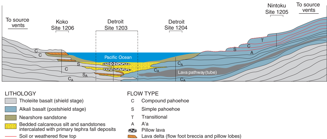
Figure 3. Schematic drawing (not to scale) showing the inferred volcanic environments for the volcanic sections drilled at Detroit (Sites 1203 and 1204), Nintoku (Site 1205) and Koko (Site 1206) Seamounts during Leg 197. The Detroit lava flows at Site 1204 and the lower part of the Site 1203 section were subaerially erupted (although shown as a submerged sequence following post-eruption subsidence). The lava flows and associated tephra fall deposits in the upper part of the Site 1203 section were emplaced into a low energy shallow marine environment. The Site 1205 lavas were entirely subaerial, as indicated by numerous soil horizons between flows. The 1206 section at Koko consists of lava flows that have flowed from land into water in a nearshore environment. Subscript "A" indicates subaerial lava emplacement.
