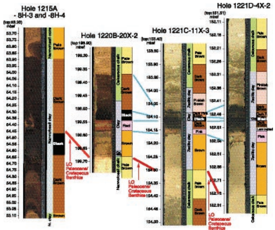
Figure 4. Paleocene-Eocene boundary sections from ODP Leg 199 (Nomura et al., 2002).
