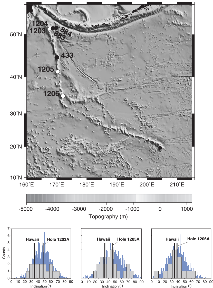
Figure 1. Top. Location of Leg 197 sites (open circles) and previous DSDP and ODP sites on the Emperor Seamounts (solid dots). The Hawaiian Islands are at the lower right. Bottom. Preliminary paleolatitudes from basaltic lava flows from Detroit Seamount (Site 1203, 35.2°), Nintoku Seamount (Site 1205, 27.1°) and Koko Guyot (Site 1206, 21.7°) are based on characteristic inclinations derived from shipboard alternating field demagnetization. The darker columns in the foreground are measured inclinations, in 5° bins; in the background are synthetic Fisherian distributions generated from the same mean and precision parameter ( k ) as the measured data. All paleolatitudes are significantly north of Hawaii, and indicate a southward motion of the hotspot, relative to the geomagnetic pole, during construction of the Emperor Seamounts.
