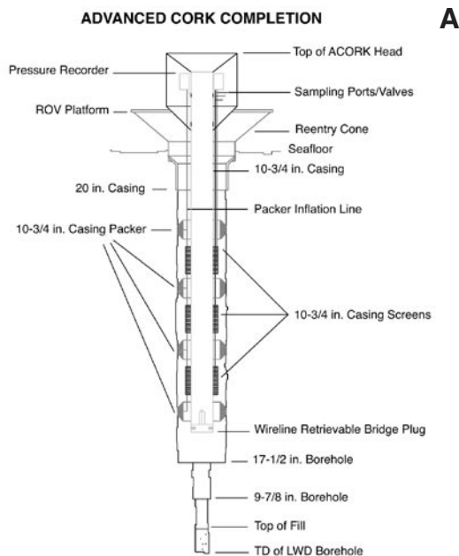
Figure 3. A. Schematic diagram of an Advanced CORK (ACORK) installed in a borehole reentry cone that has 20 in and 10-3/4 in casing set in the hole (after Graber et al. 2002). Downhole external 10-3/4 in casing packers seal off zones of open hole between external screened sampling sections and below the casing. Screened sections are connected by hydraulic sampling tubing to valves and ports in the ACORK head that sits above the reentry cone and submersible platform; the head contains hydraulic and pressure sampling devices and provides access for downloading data. B. ACORK installed at Hole 1173B in the Nankai Trough off Japan during ODP Leg 196 in 2001. The reentry cone was set at the end of initial drilling during ODP Leg 190 in 2000. The basket of the ROV Kaiko is visible in front of the ACORK head in this image taken during a 2002 data collection dive (Video still courtesy of JAMSTEC).
