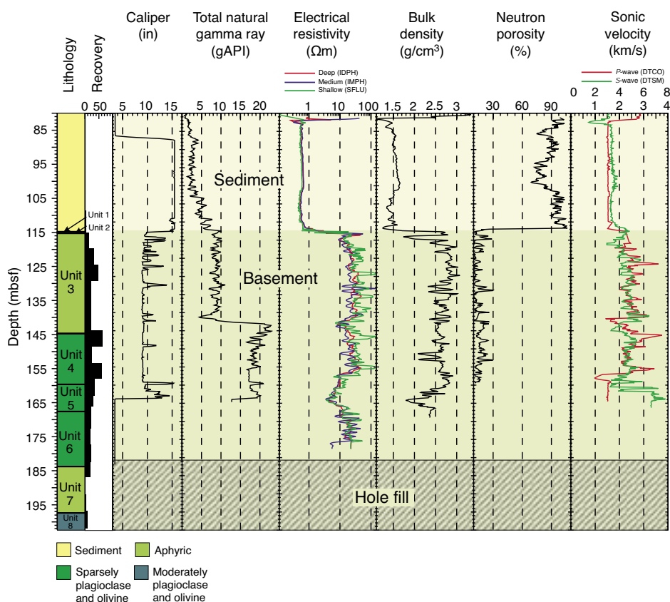
Figure 2. Composite plot of down-hole measurements in the sediment and basement section of Hole 1243B. Note that log depths are based on wireline measurements, whereas core depths are based on drill pipe measurements. The core lithology has been shifted down 6.3 m to match the logging-derived depths. GAPI= American Petroleum Institute gamma ray units ( Orcutt, Schultz, Davies et al., 2003).
