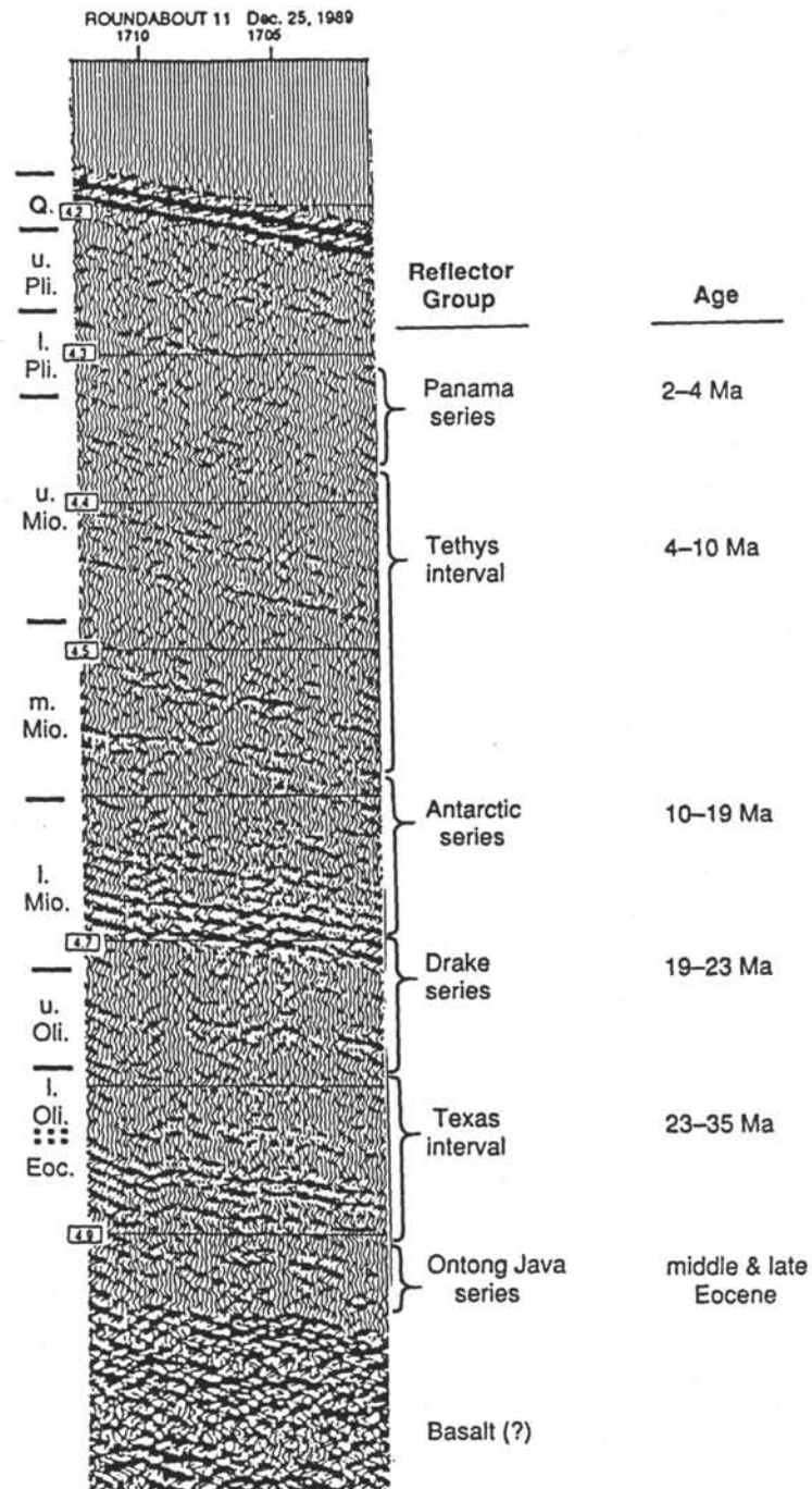
Figure 15. Seismic profile at Site 805, taken by R/V Thomas Washington on Cruise ROUNDABOUT 11, with time-scale assigned from drilling and logging results. Two-way travel time indicated on left-hand side of figure. Names to the right refer to distinct groups of reflectors ("series") and to zones with no distinct groups of reflectors ("intervals"). Three of the names are taken from suggestions by Mayer et al. (1986) regarding the origin of such reflectors (Panama, Antarctic, Drake Passage). While these hypotheses are appealing, our use of these names does not imply that we consider them approved. For "Tethys" and "Texas" intervals, see text.
