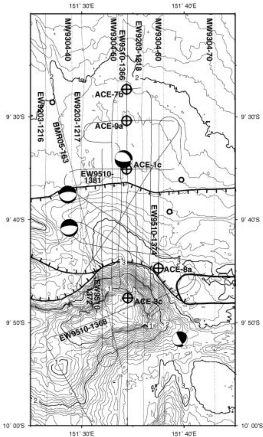
FIG. 3 MCS track chart on a 100 m bathymetry base with the proposed drill sites (ACE-1c, 3c, 7b, 8a, 9a). Black circles are relocated epicenters, which together with the focal mechanisms, are from Abers et al (1997). The western limit of the Woodlark spreading system is marked by the closed black line, major normal faults by the ticked lines.
